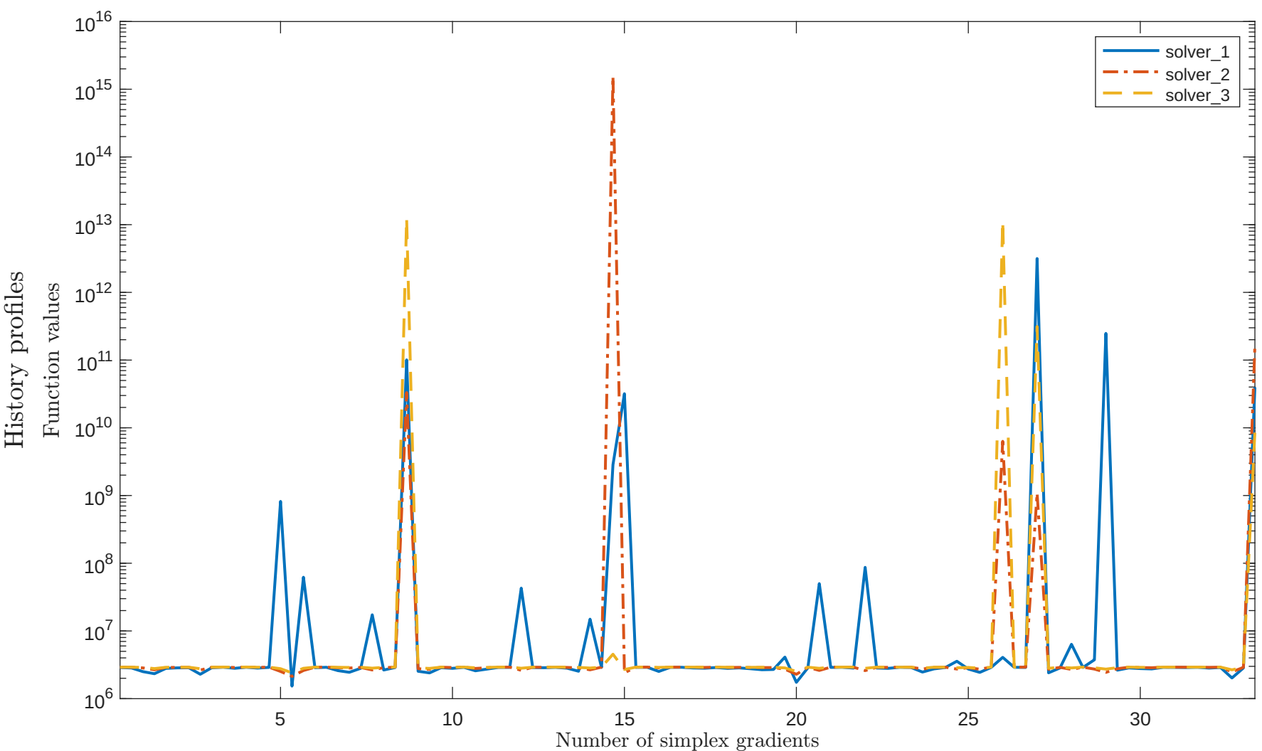
Solving "MISRA1BLS" with "plain" feature
