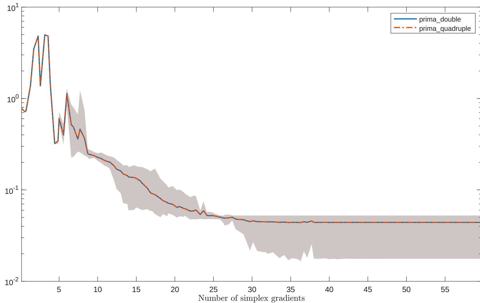
Solving "BIGGS6" with "noisy_0.001_mixed-gaussian" feature
