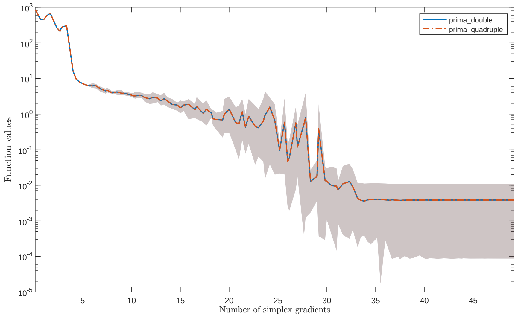
Solving “CHNROSNB” with “noisy_0.001_mixed-gaussian” feature
