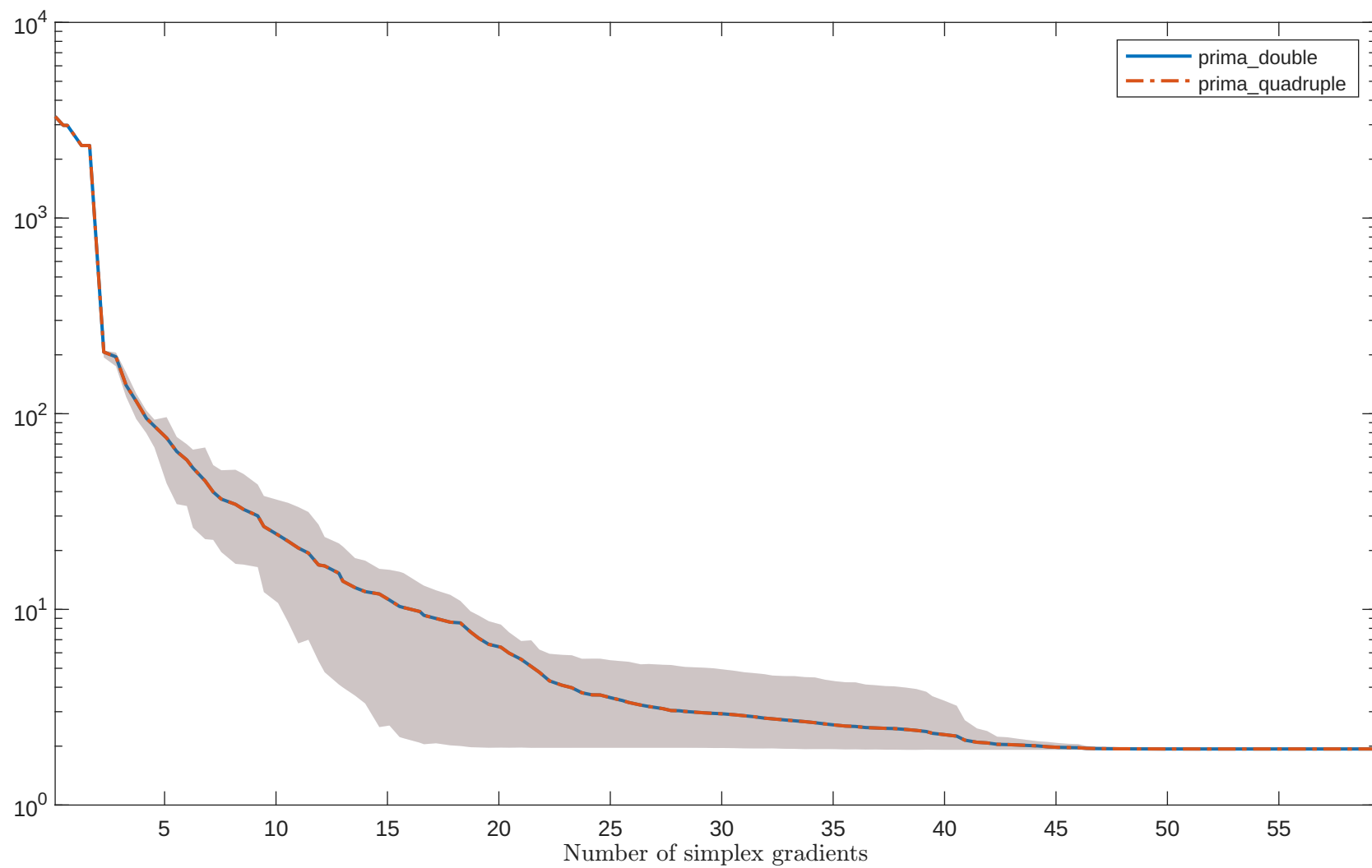
Solving “Cragglvy” with “noisy_0.001_mixed_gaussian” feature
