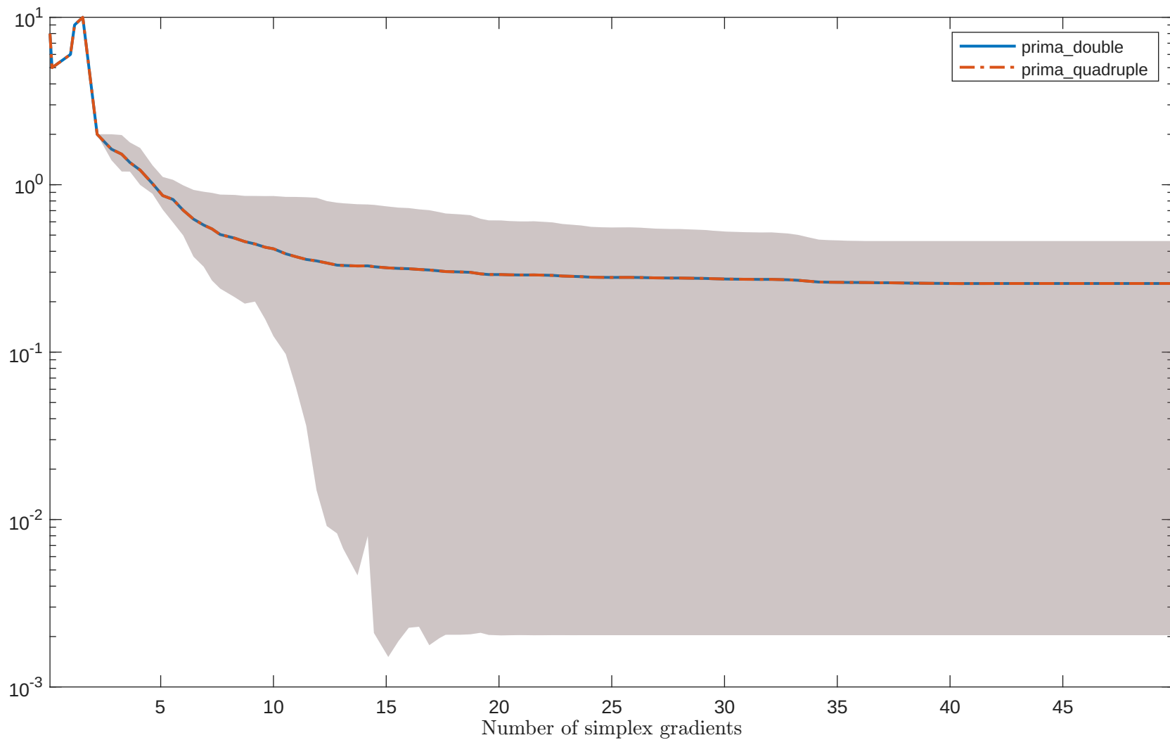
Solving “DIXON3DQ” with “noisy_0.001_mixed_gaussian” feature
