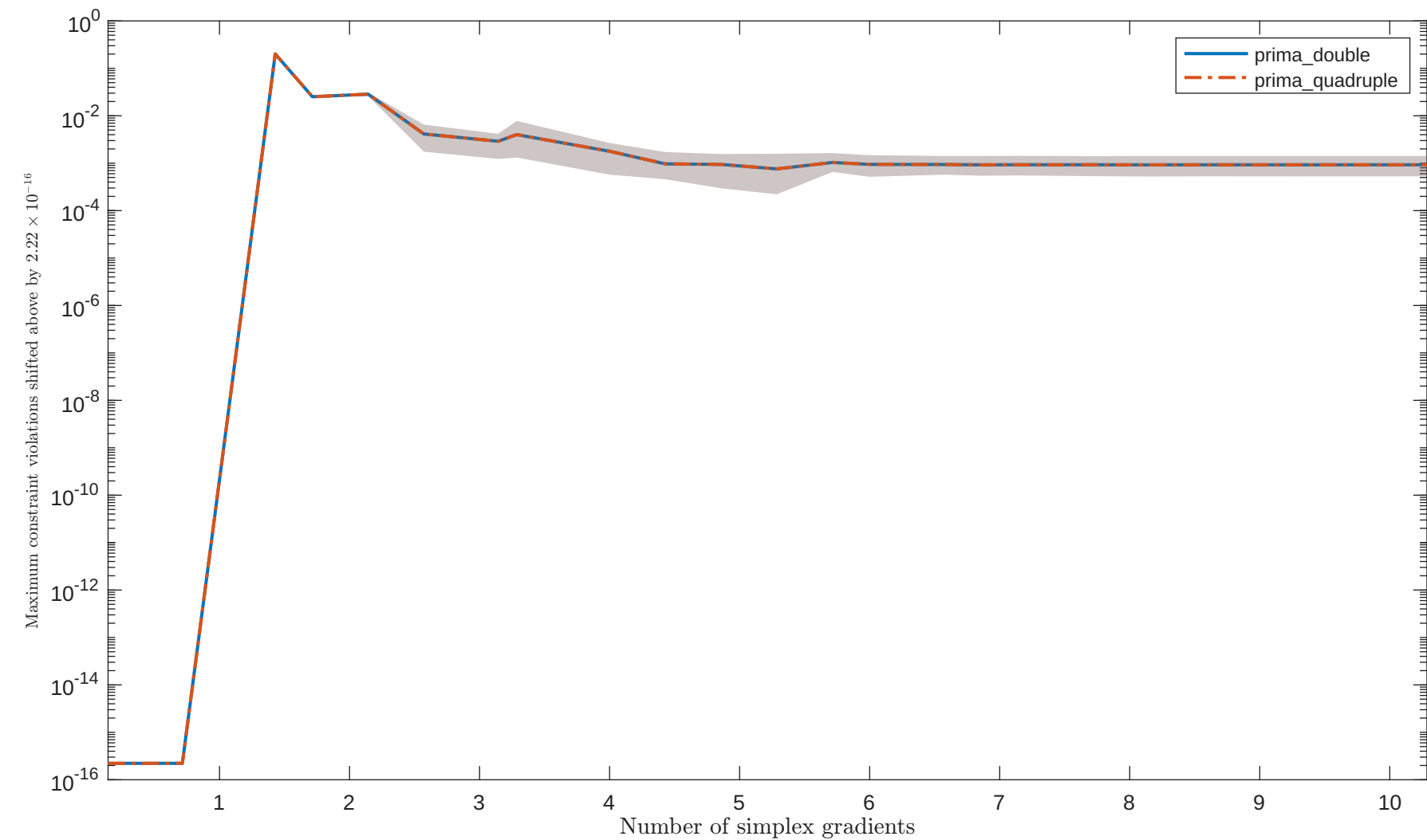
Solving "EIGENACO" with "noisy_0.001_mixed_gaussian" feature
