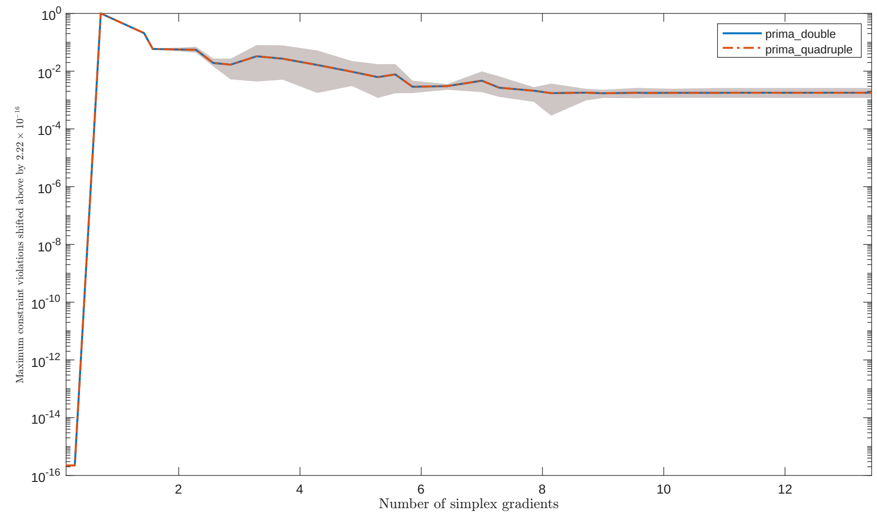
Solving "EIGENB2" with "noisy_0.001_mixed-gaussian" feature
