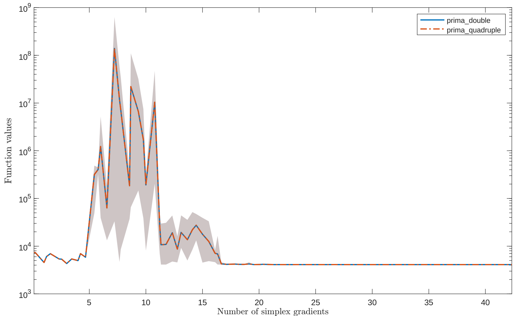
Solving “GAUSS1LS” with “noisy_0.001_mixed_gaussian” feature
