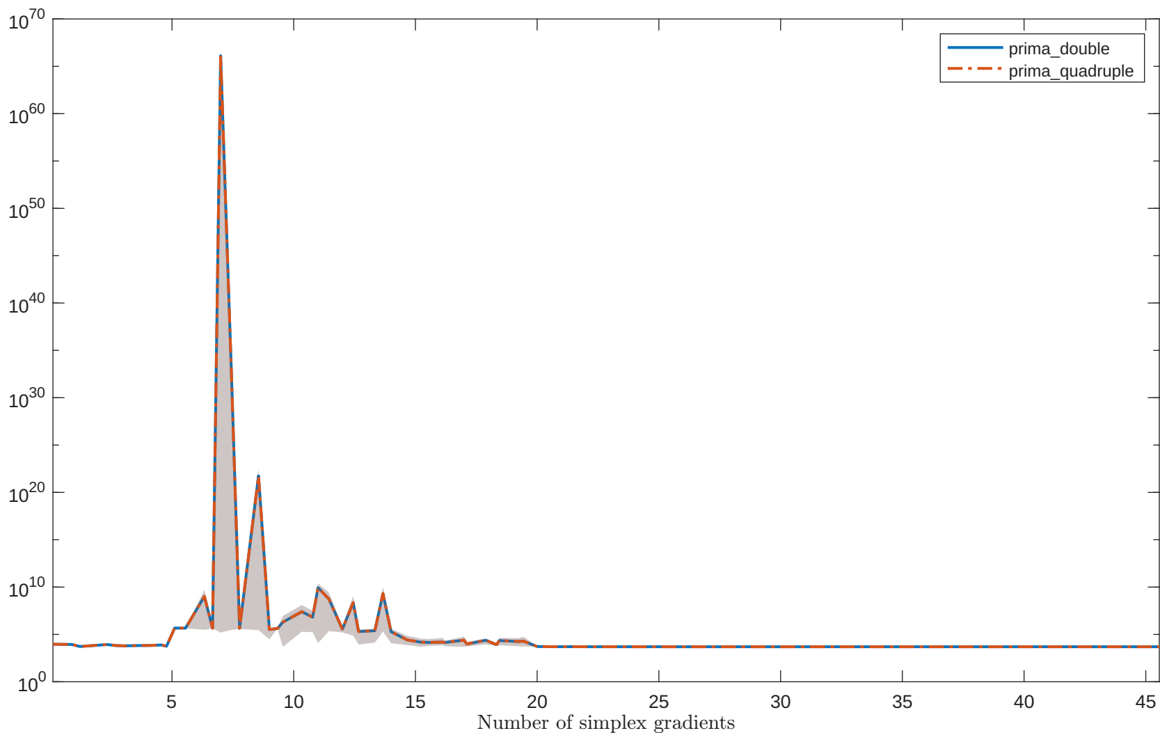
Solving “GAUSS2LS” with “noisy_0.001_mixed_gaussian” feature
