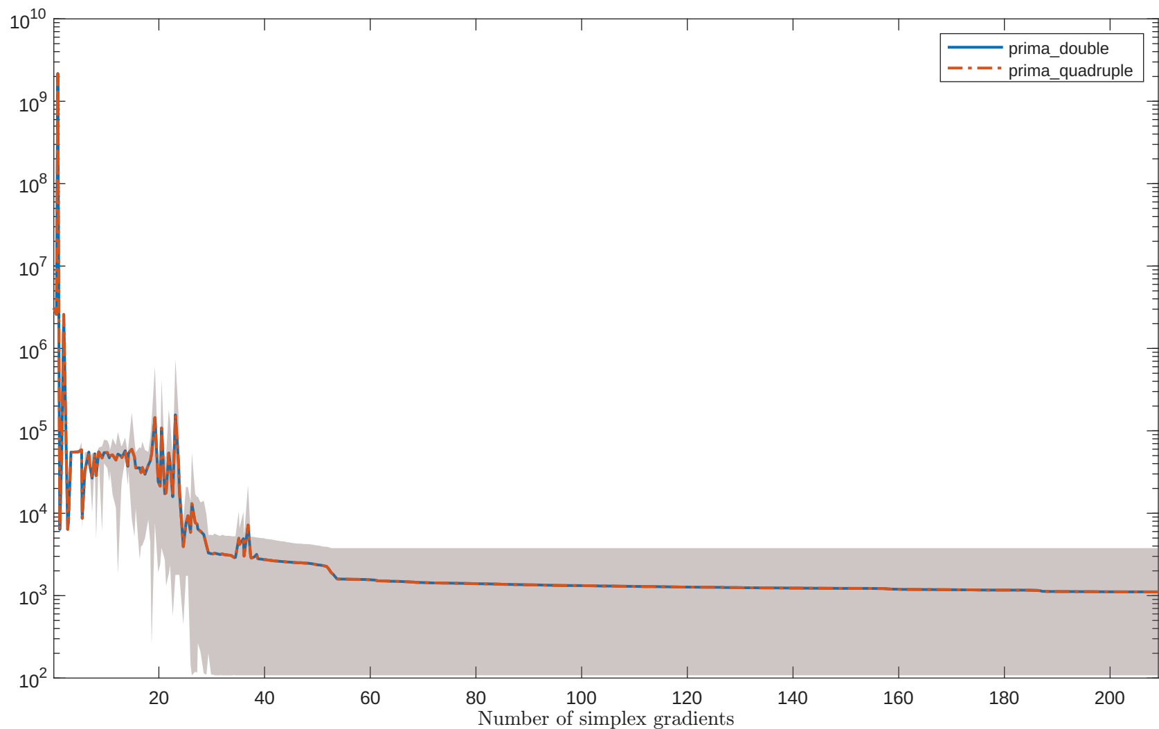
Solving “HAHN1LS” with “noisy_0.001_mixed_gaussian” feature
