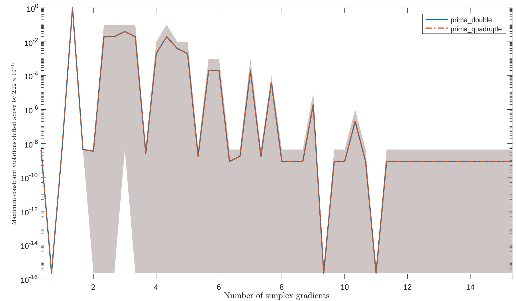
Solving "HS21" with "noisy_0.001_mixed_gaussian" feature
