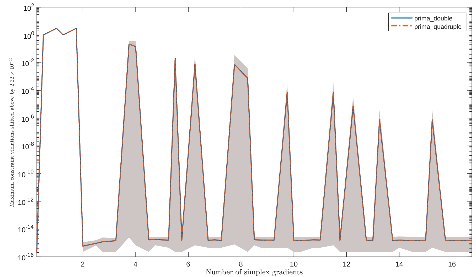
Solving "HS28" with "noisy_0.001_mixed_gaussian" feature
