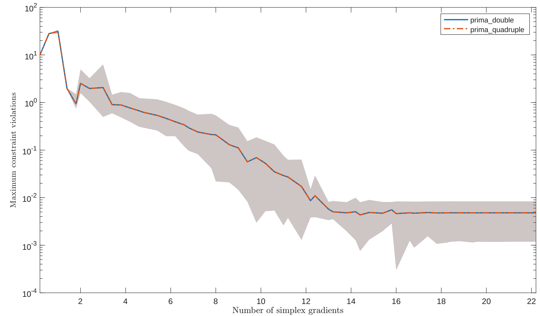
Solving “HS39” with “noisy_0.001_mixed.gaussian” feature
