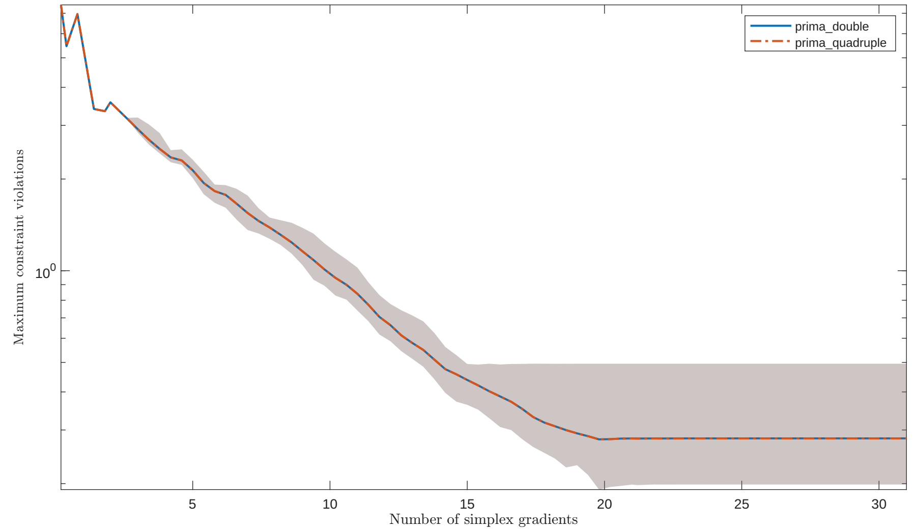
Solving “HS72” with “noisy_0.001_mixed-gaussian” feature
