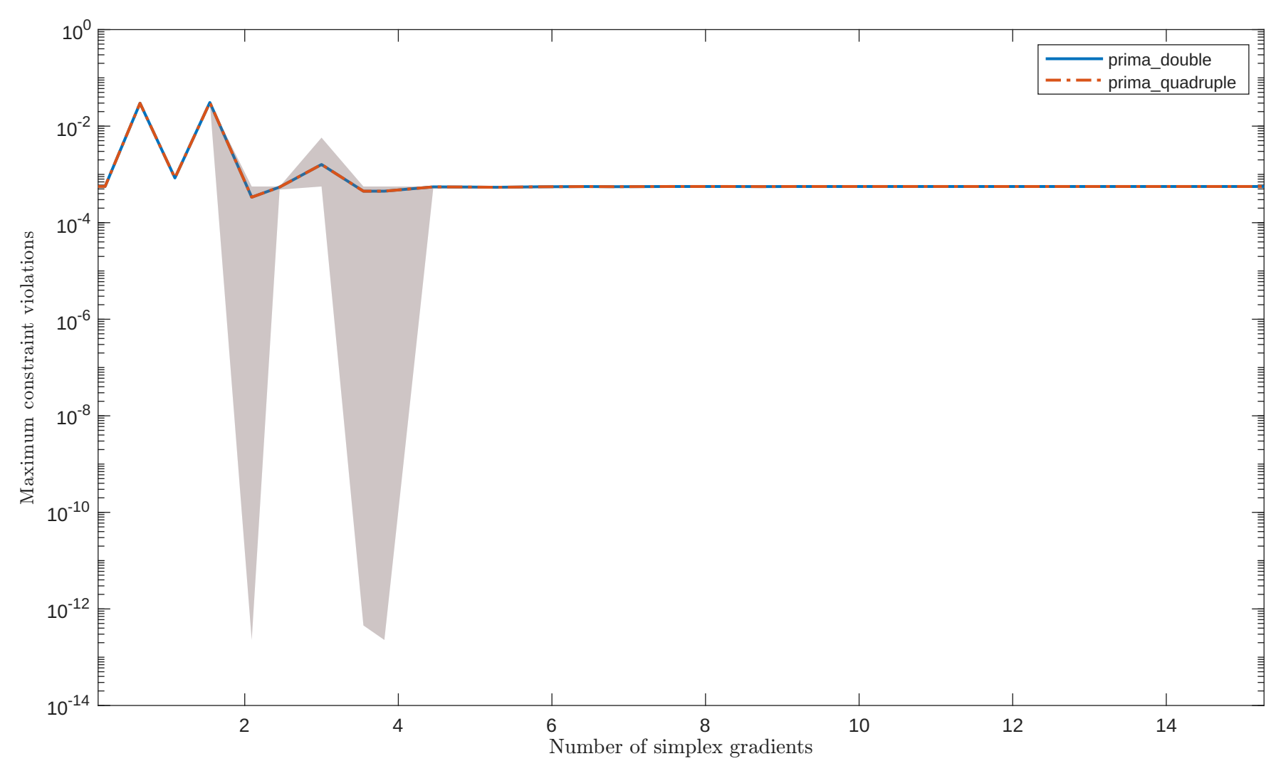
Solving “HUESmMOD” with “noisy_0.001_mixed_gaussian” feature
