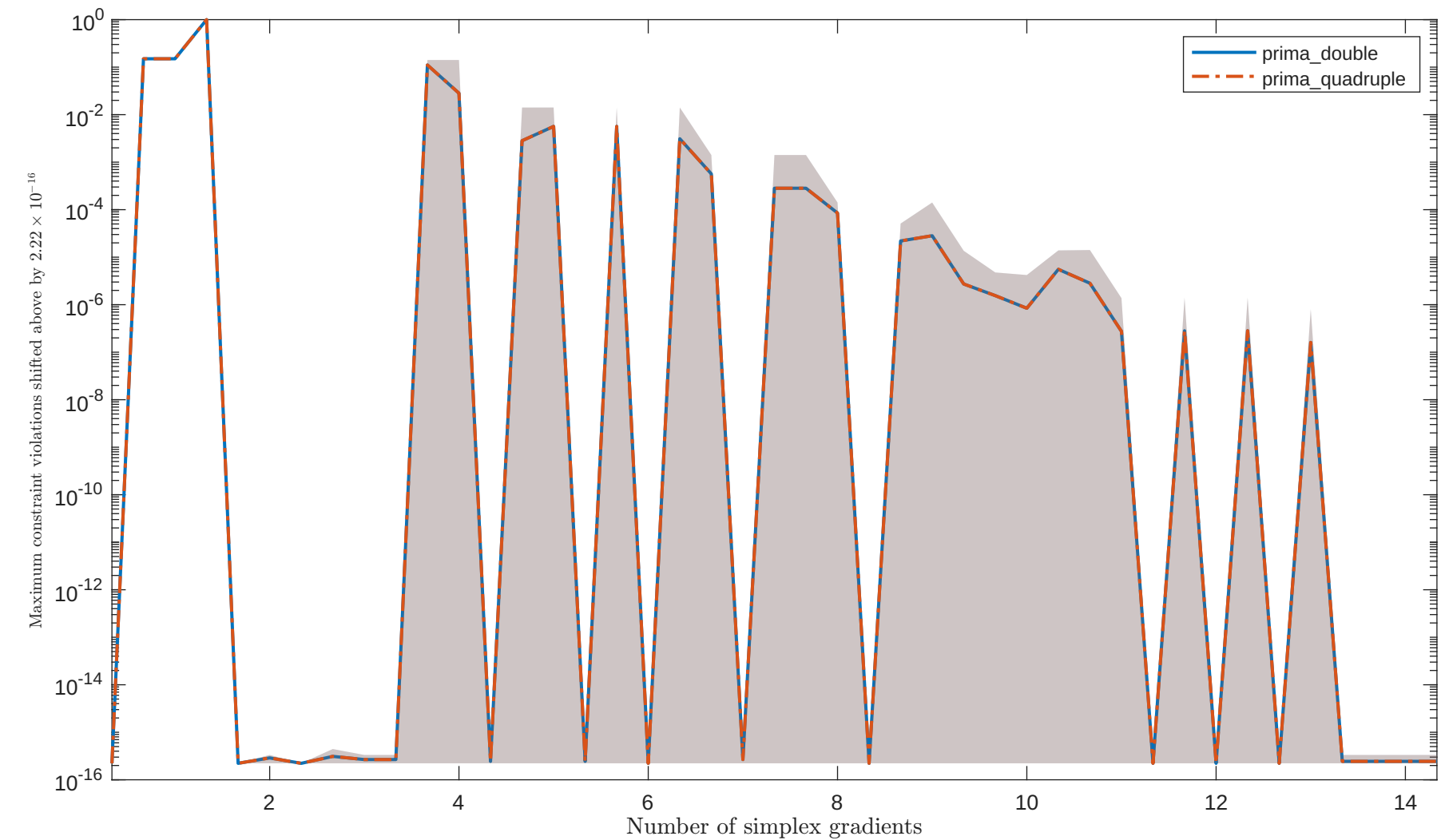
Solving “LSQFIT” with “noisy_0.001_mixed_gaussian” feature
