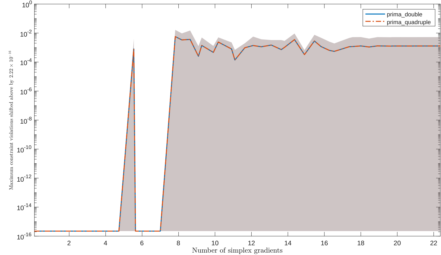
Solving “LUKVLI3” with “noisy_0.001_mixed_gaussian” feature
