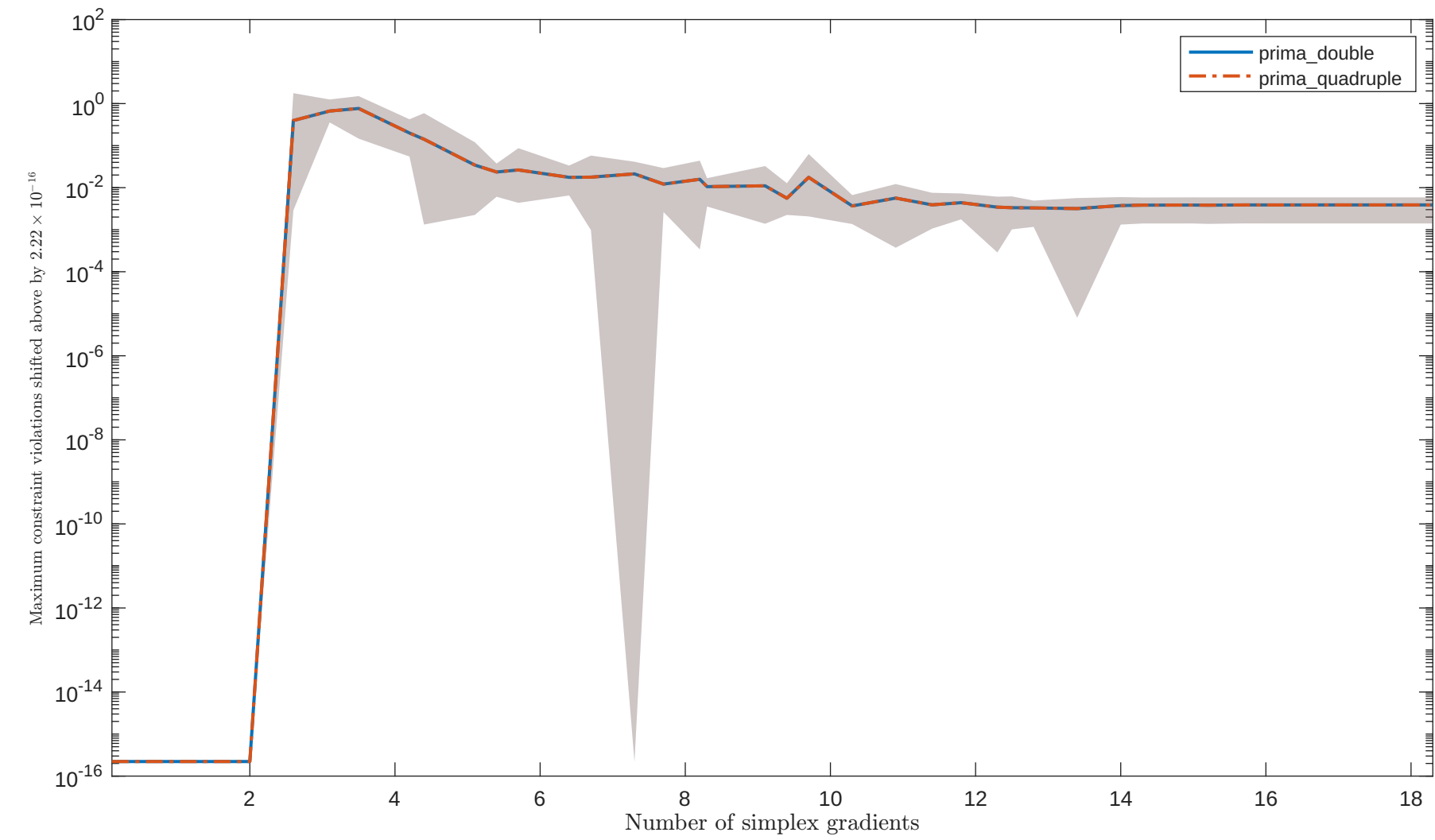
Solving “LUKVL16” with “noisy_0.001_mixed_gaussian” feature
