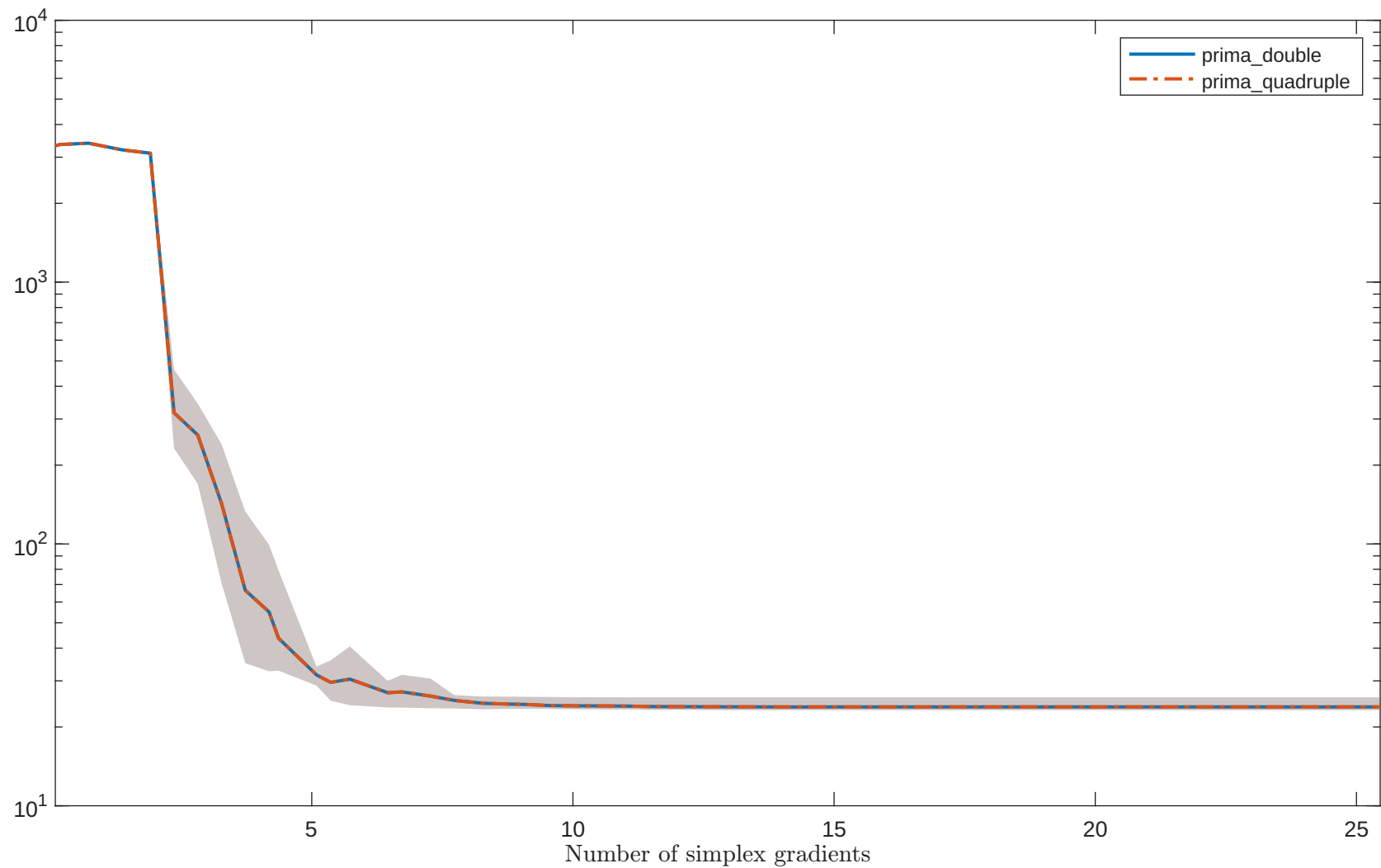
Solving “NONCVXUN” with “noisy_0.001_mixed_gaussian” feature
