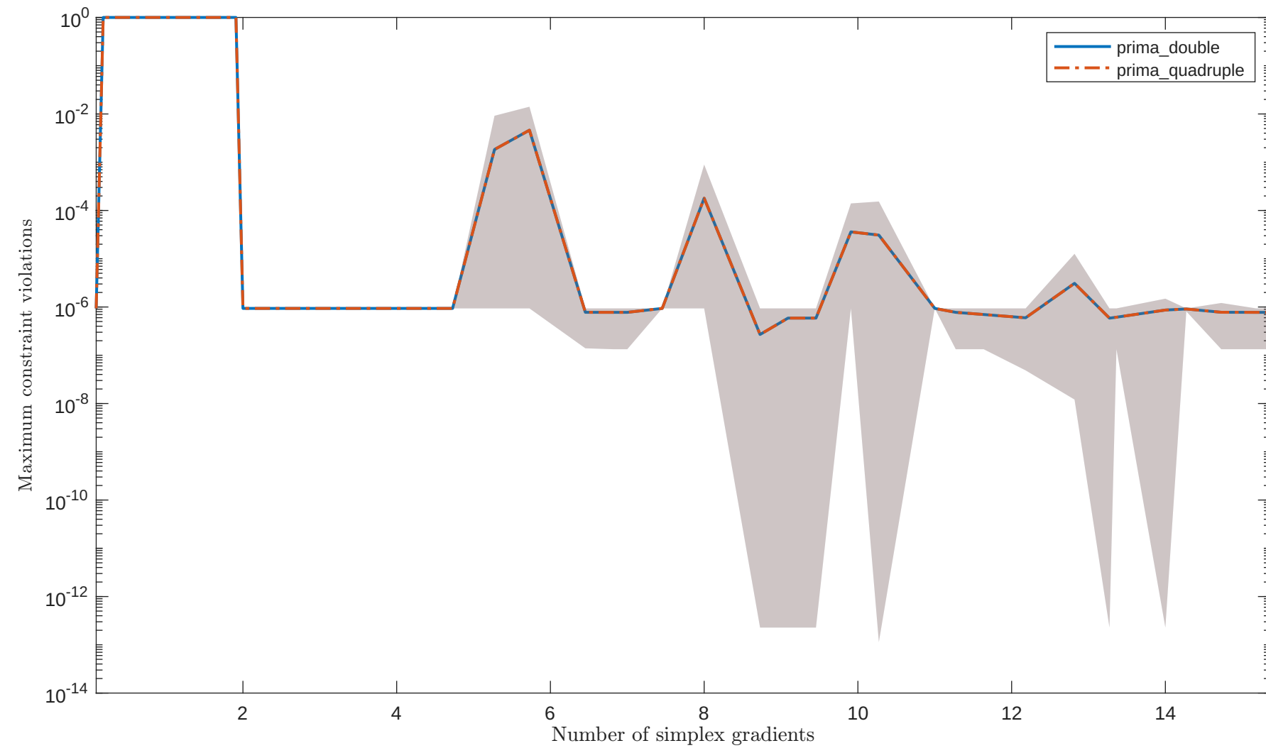
Solving “ODFITS” with “noisy_0.001_mixed.gaussian” feature
