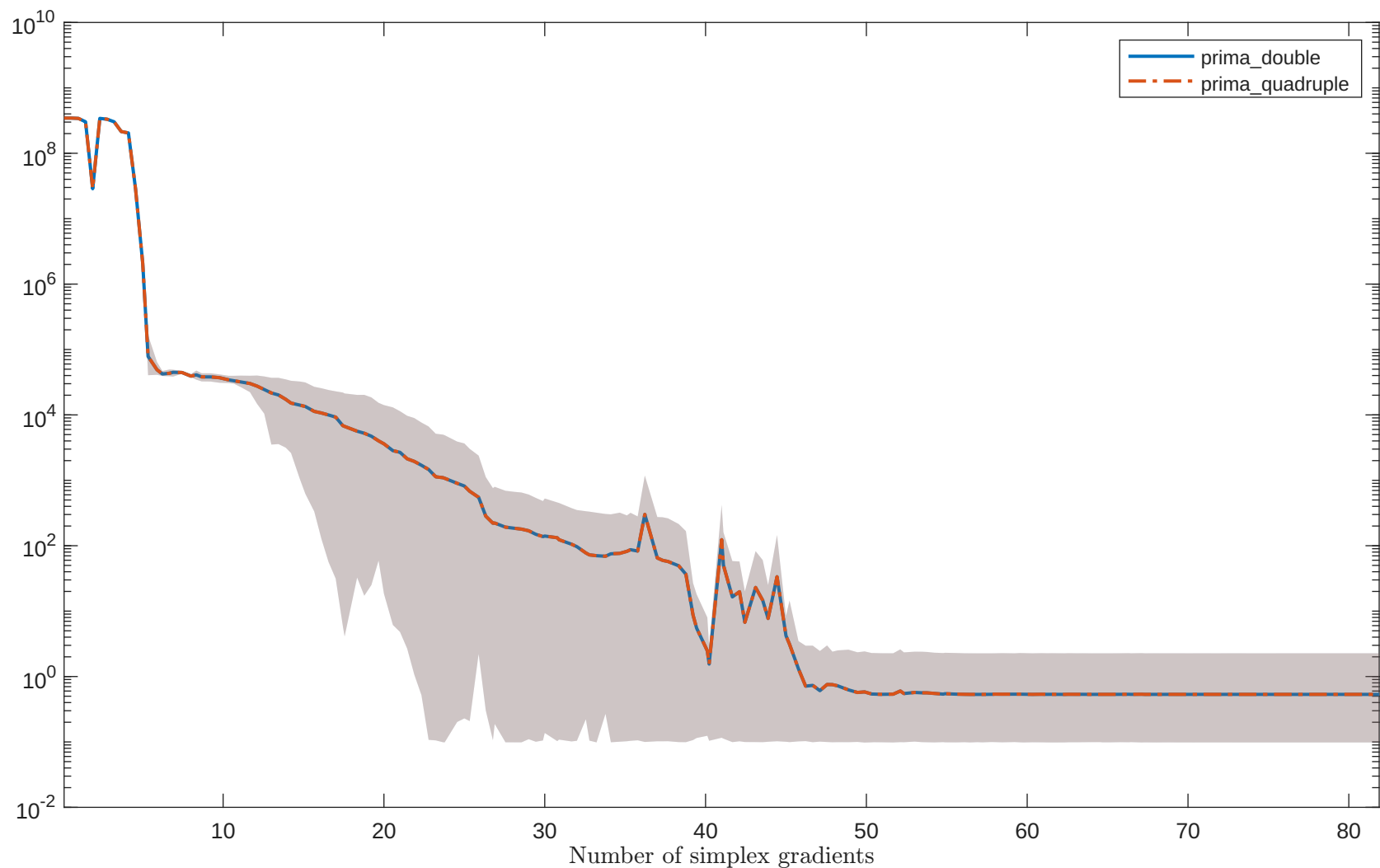
Solving “PALMER1C” with “noisy_0.001_mixed_gaussian” feature
