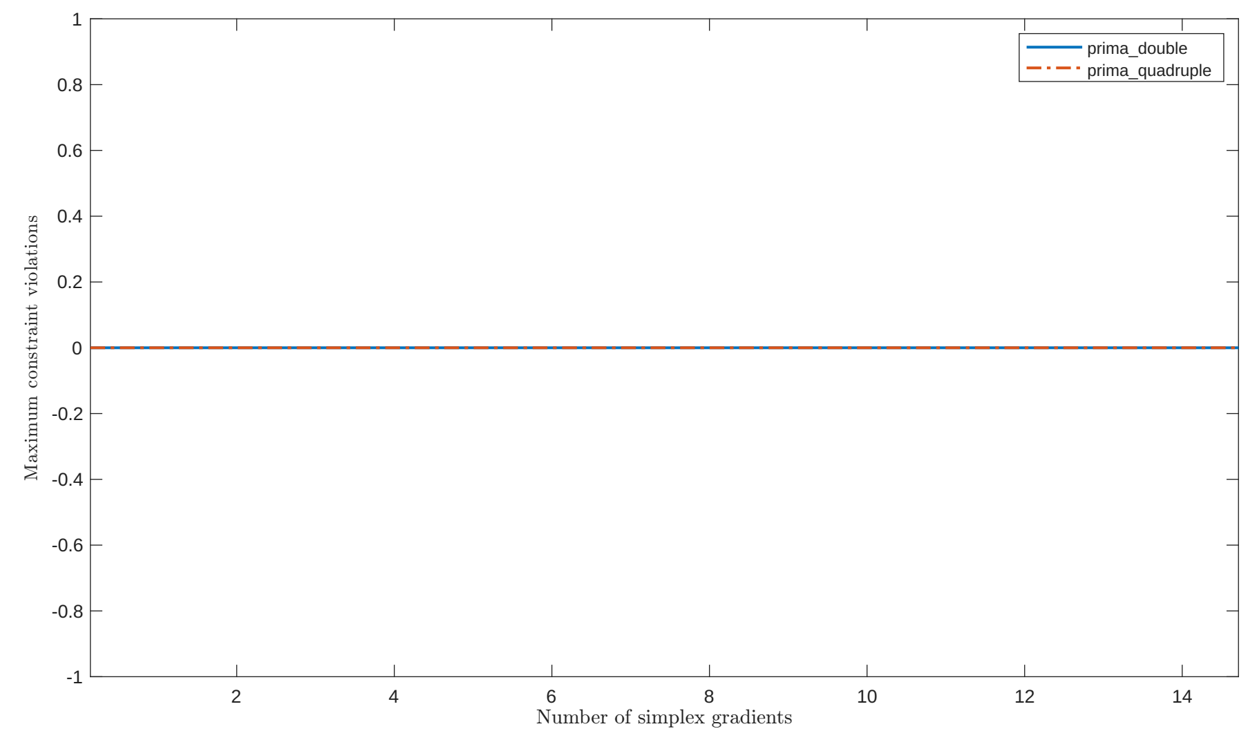
Solving "PALMER2A" with "noisy_0.001_mixed_gaussian" feature
