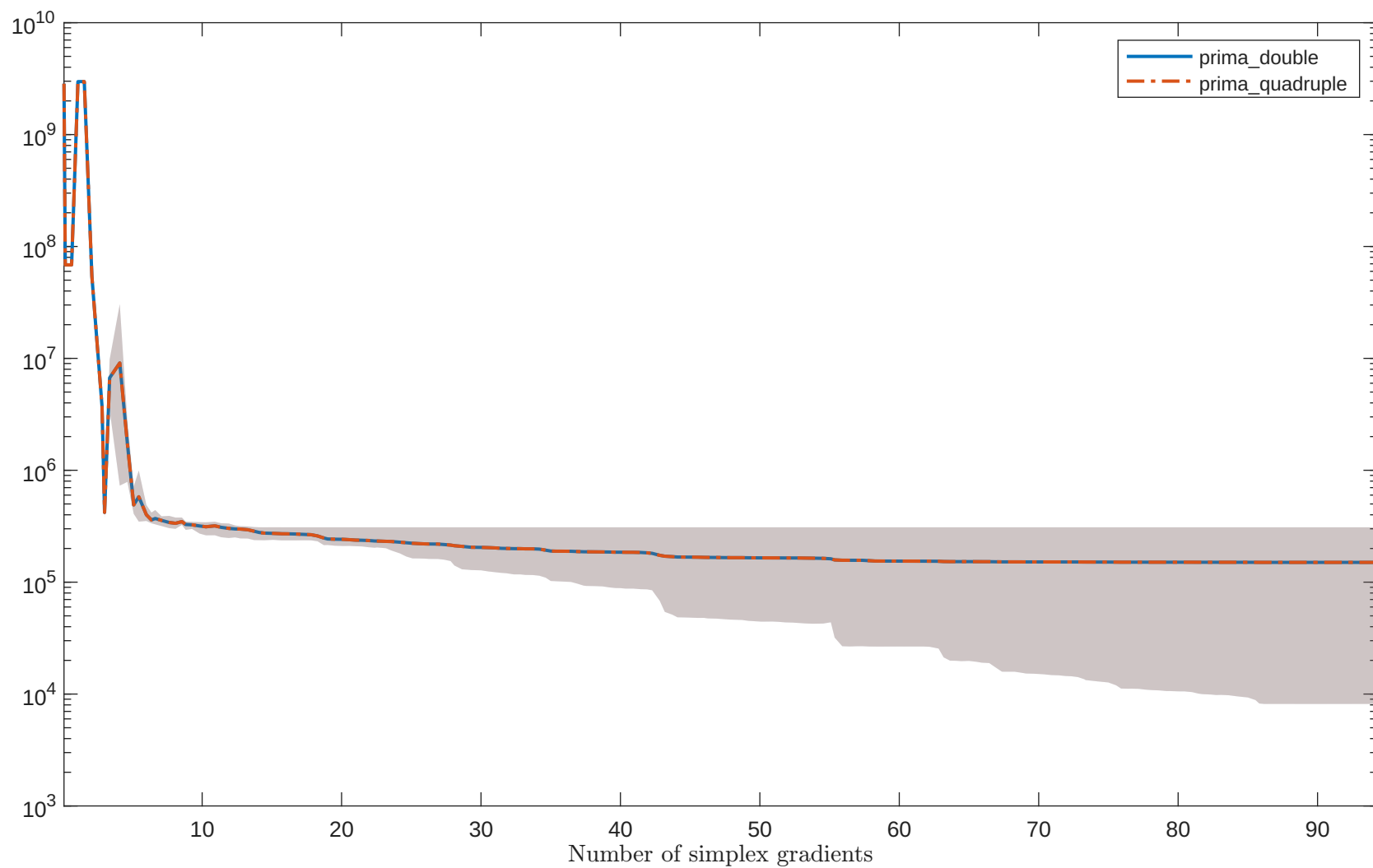
Solving "POWERSUM" with "noisy_0.001_mixed_gaussian" feature
