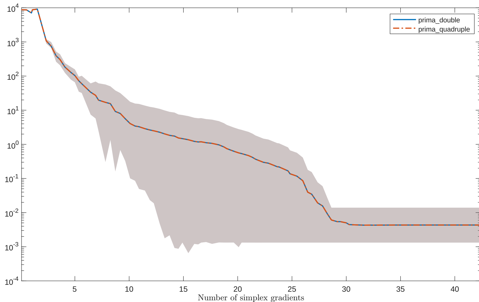
Solving “QUARTC” with “noisy_0.001_mixed_gaussian” feature
