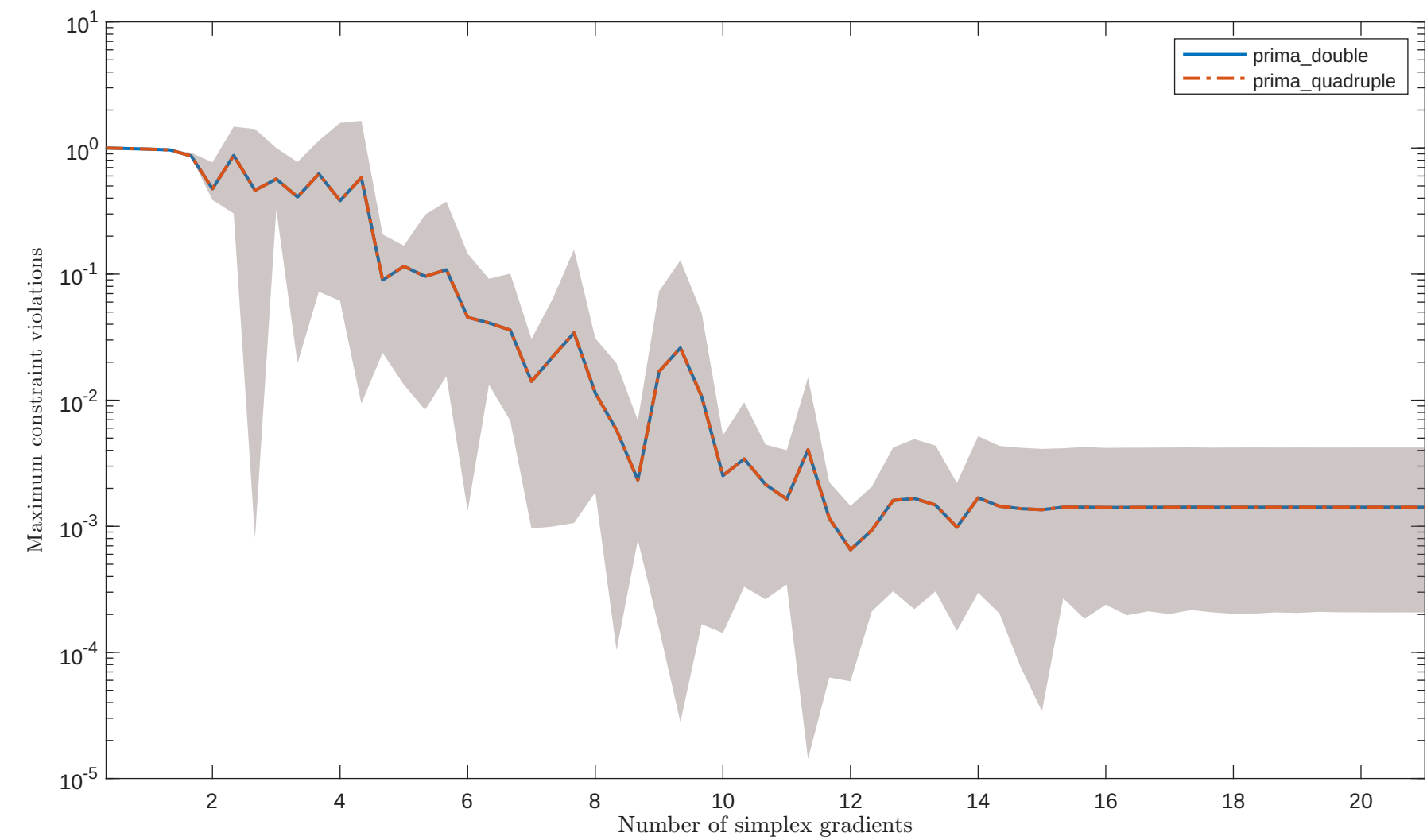
Solving "S316m322" with "noisy_0.001_mixed_gaussian" feature
