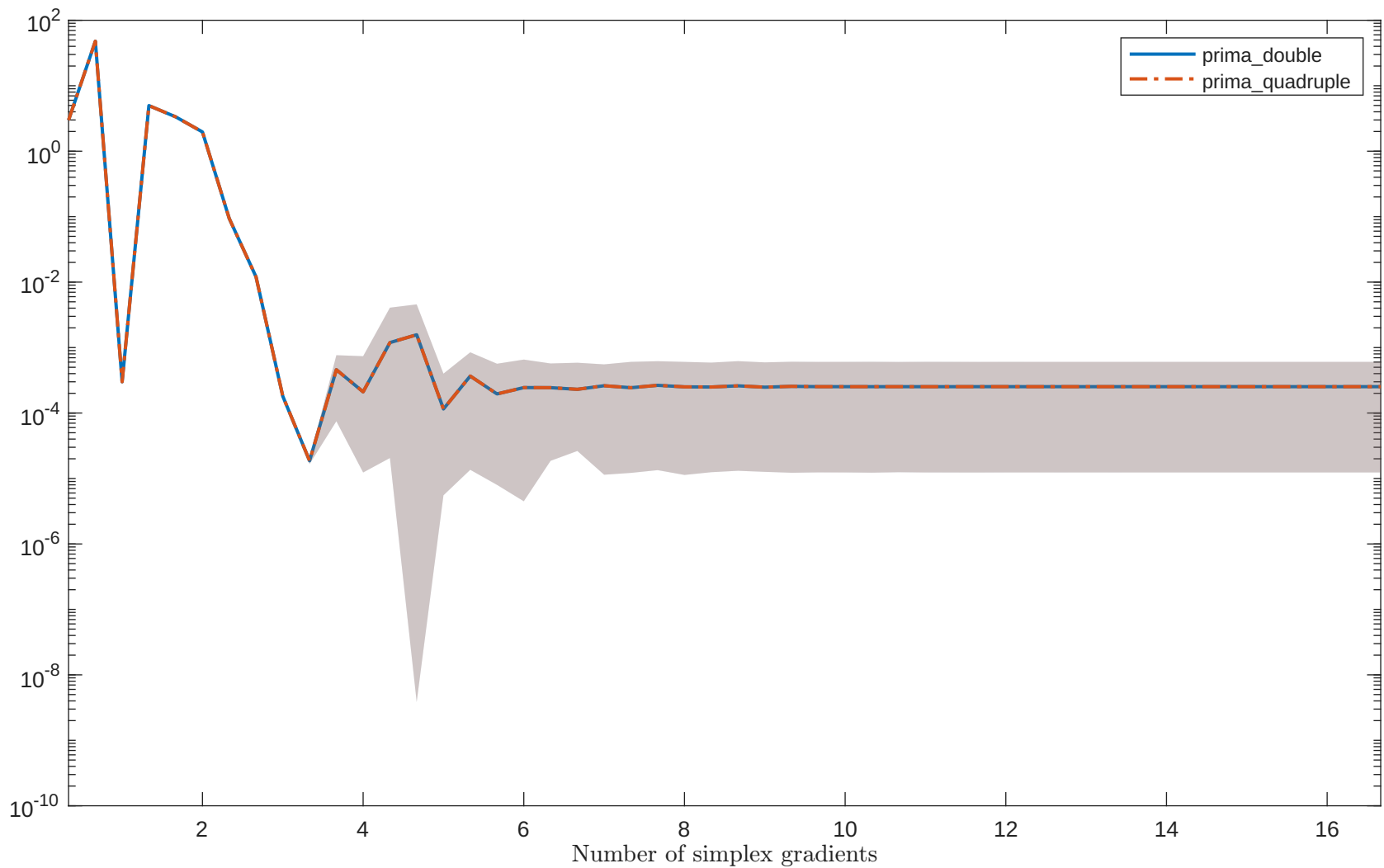
Solving "SISSER2" with "noisy_0.001_mixed_gaussian" feature
