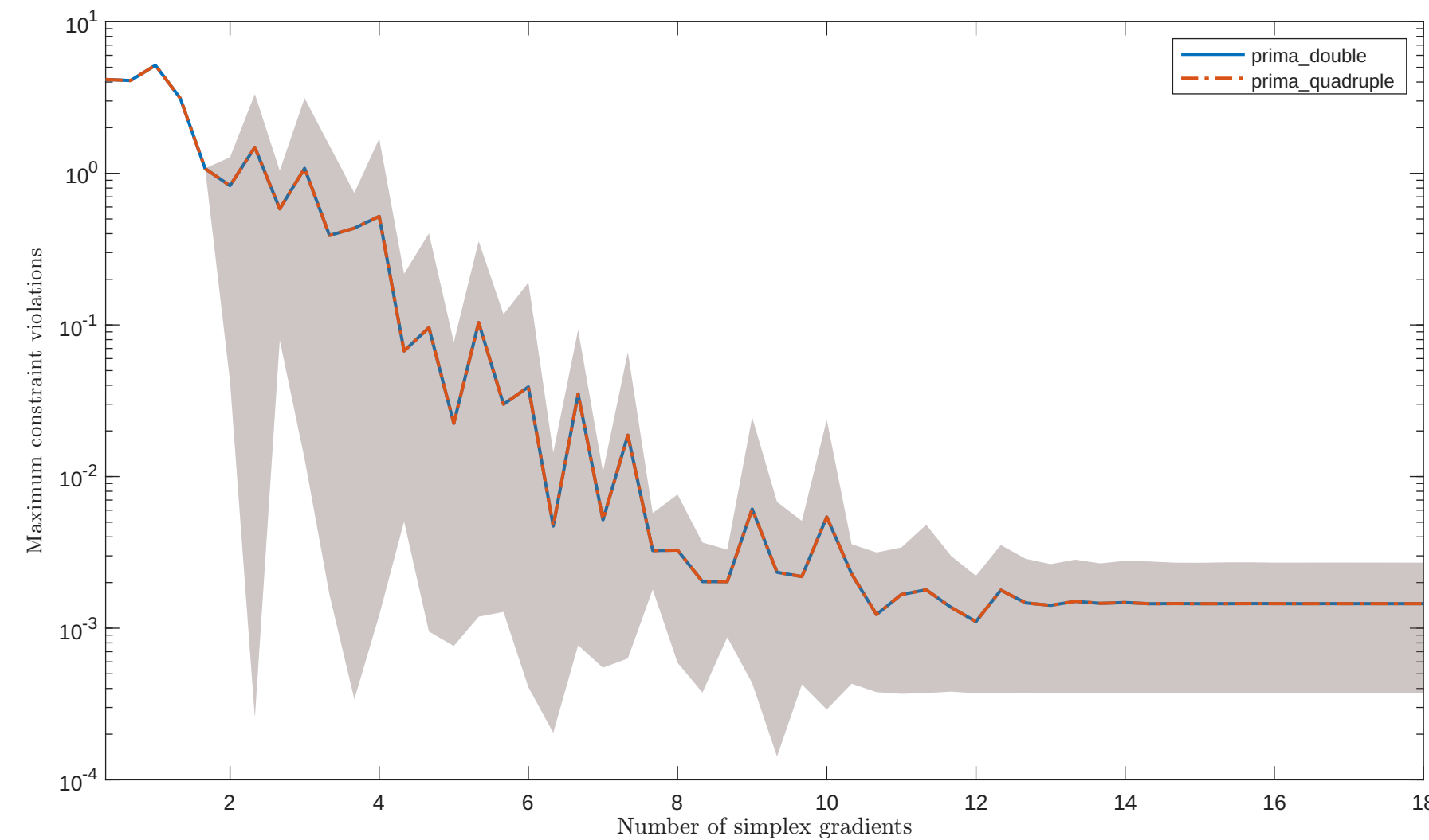
Solving "SNAKE" with "noisy_0.001_mixed_gaussian" feature
