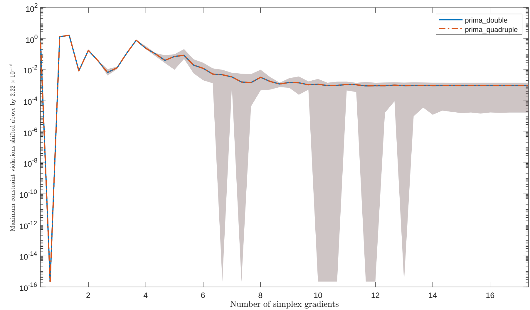
Solving "TWOBARS" with "noisy_0.001_mixed_gaussian" feature
