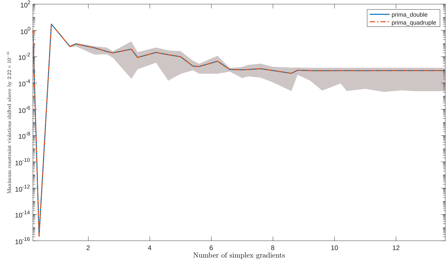
Solving “HS42” with “noisy_0.001_mixed_gaussian” feature
