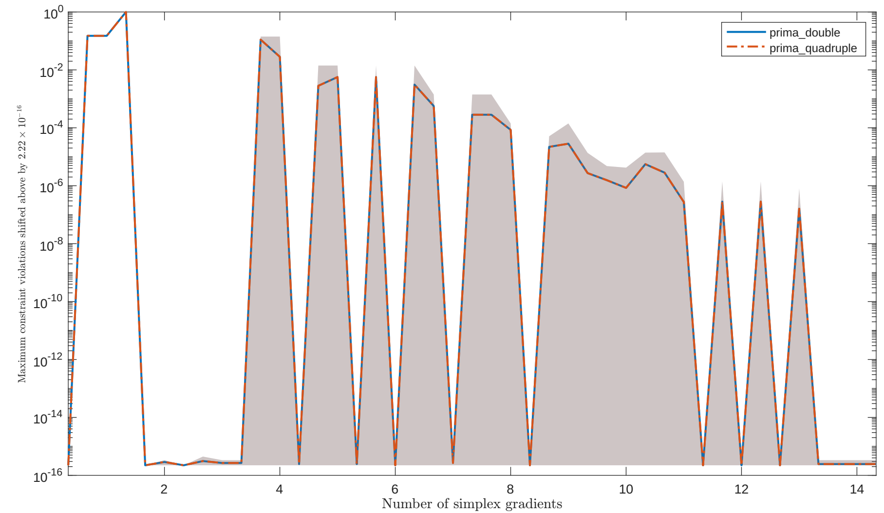
Solving “LSQFIT” with “noisy_0.001_mixed_gaussian” feature
