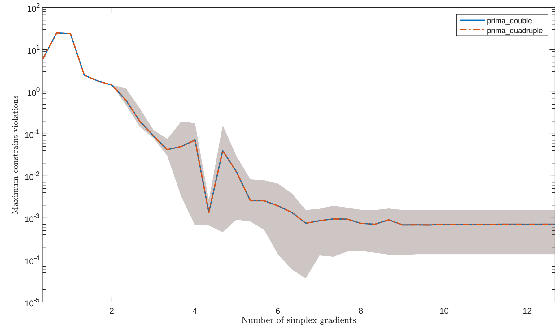
Solving "BT10" with "noisy_0.001_mixed.gaussian" feature
