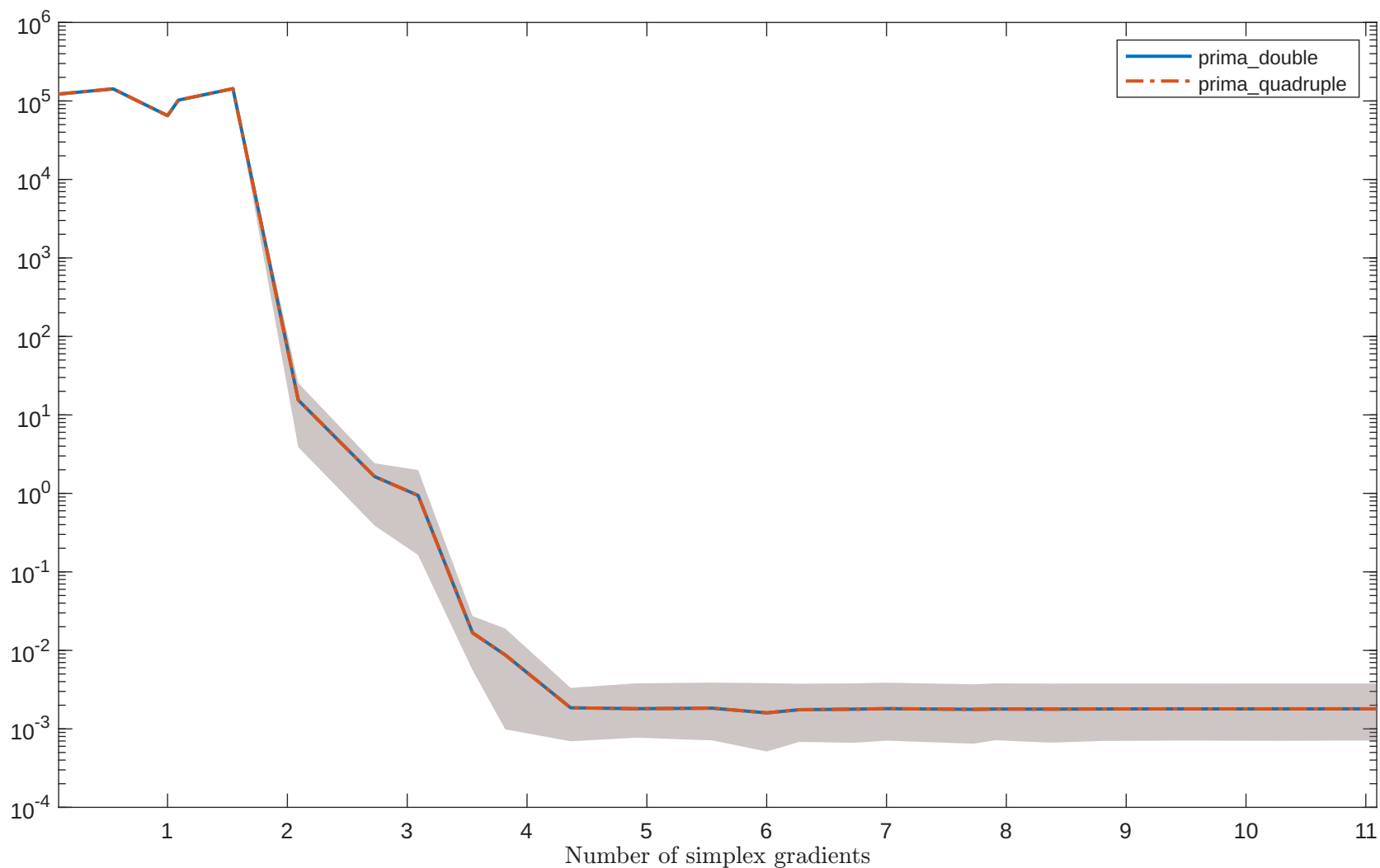
Solving “MANCINO” with “noisy_0.001_mixed_gaussian” feature
