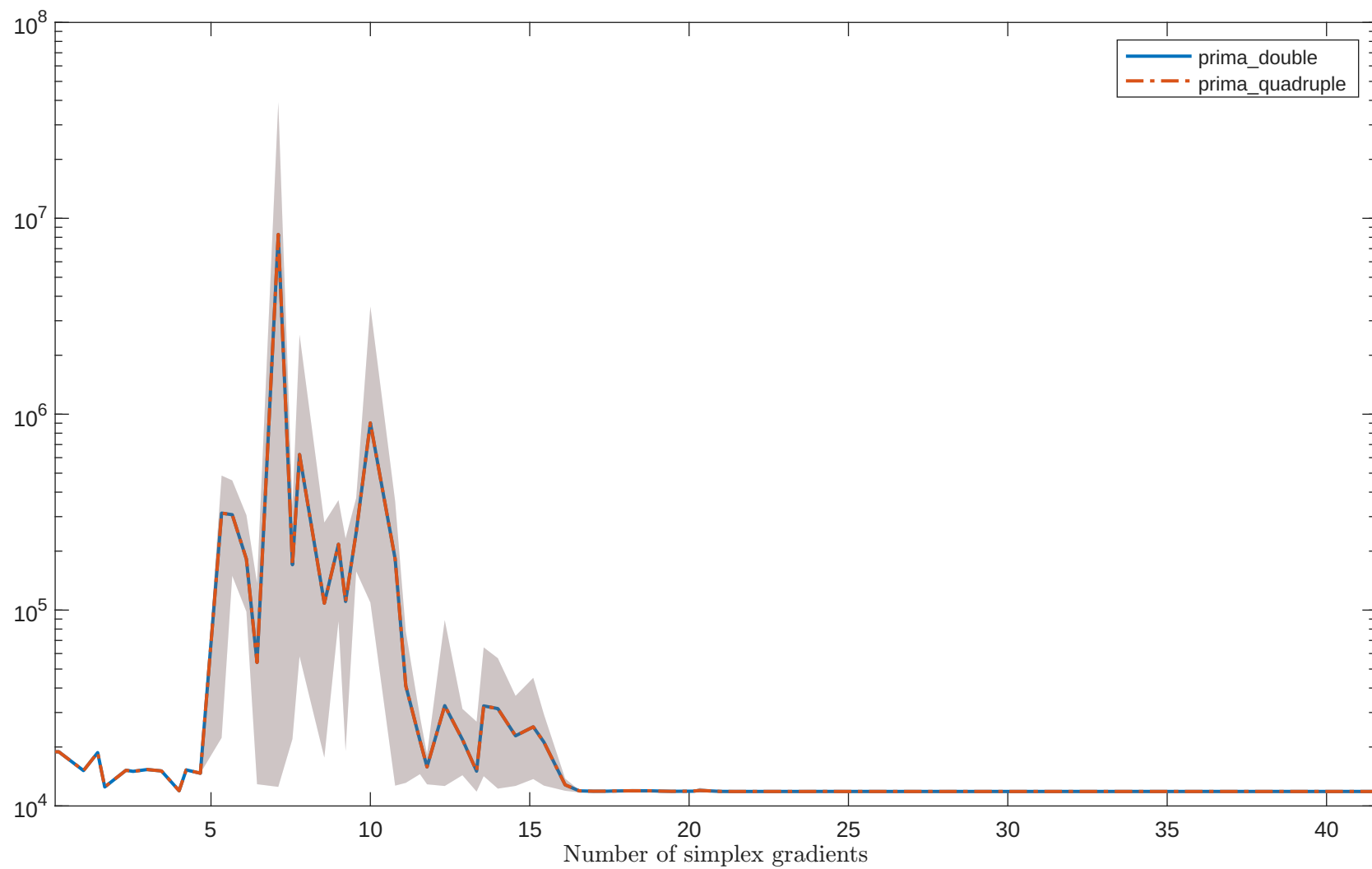
Solving “GAUSS3LS” with “noisy_0.001_mixed_gaussian” feature
