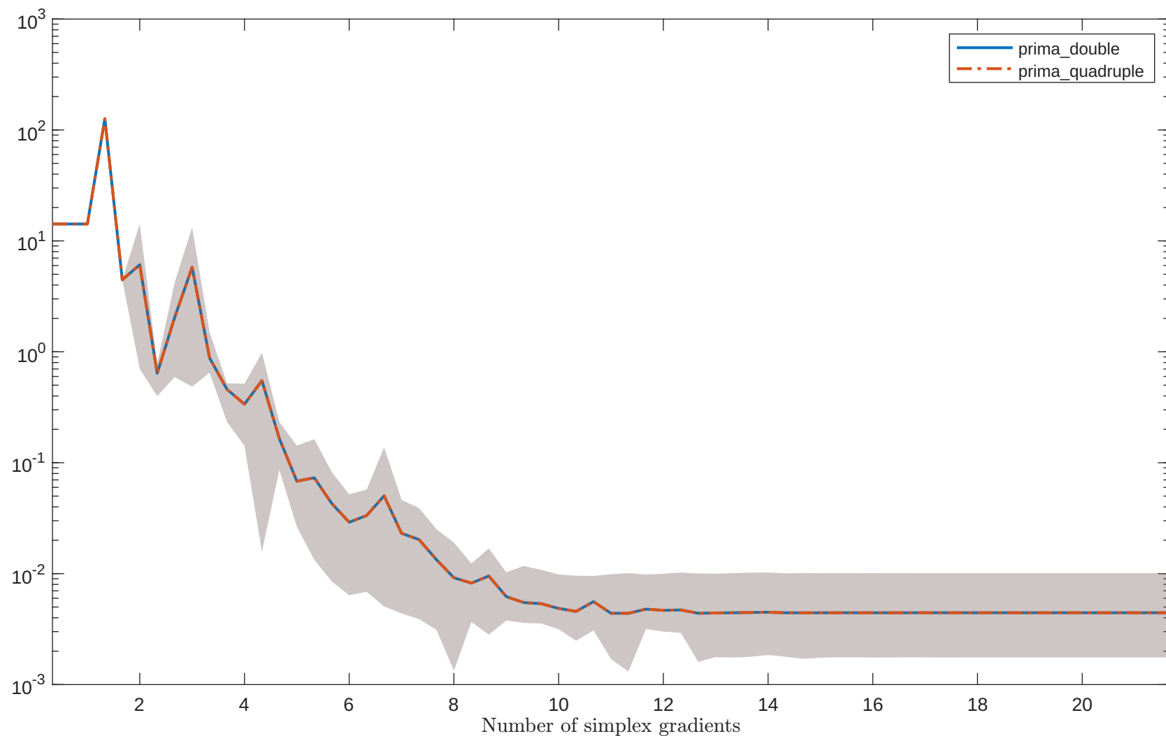
Solving “BEALE” with “noisy_0.001_mixed_gaussian” feature
