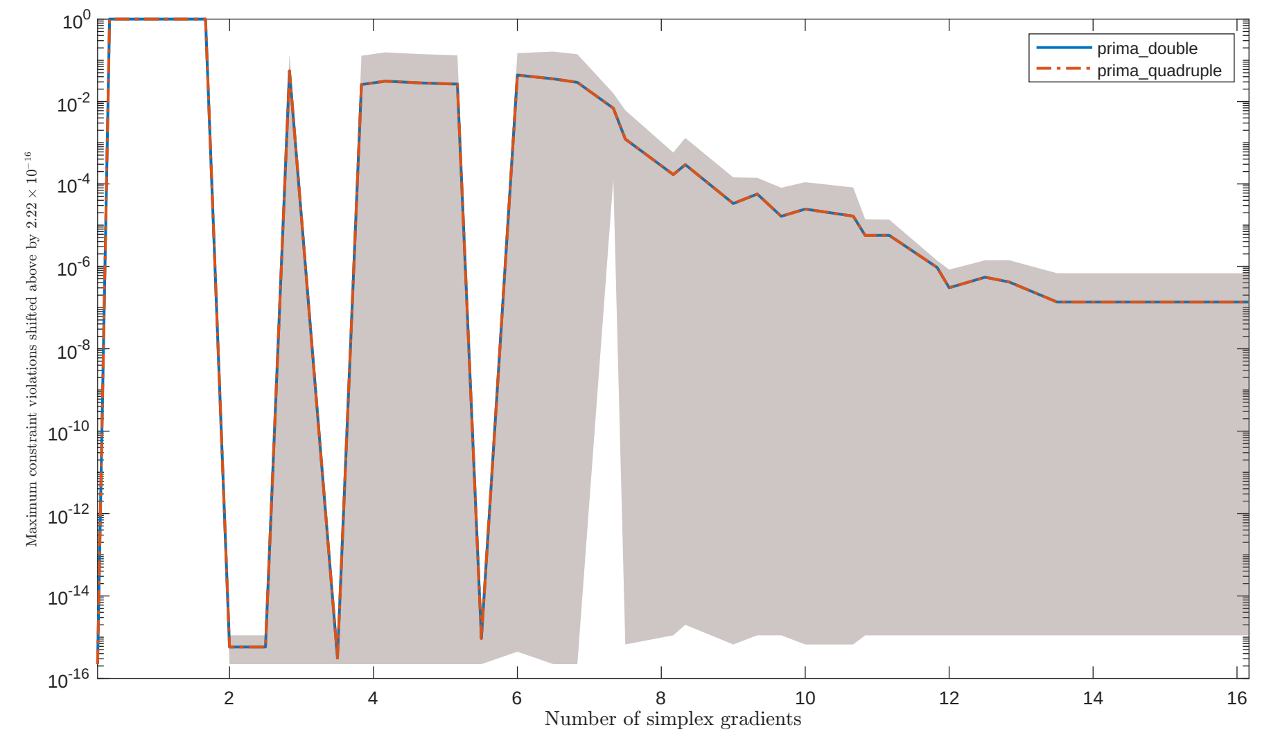
Solving "LSNNODOC" with "noisy_0.001_mixed_gaussian" feature
