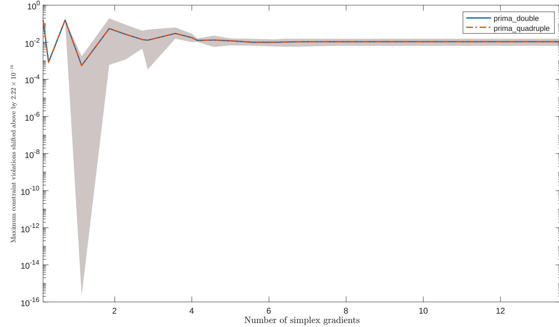
Solving "HS90" with "noisy_0.001_mixed_gaussian" feature
