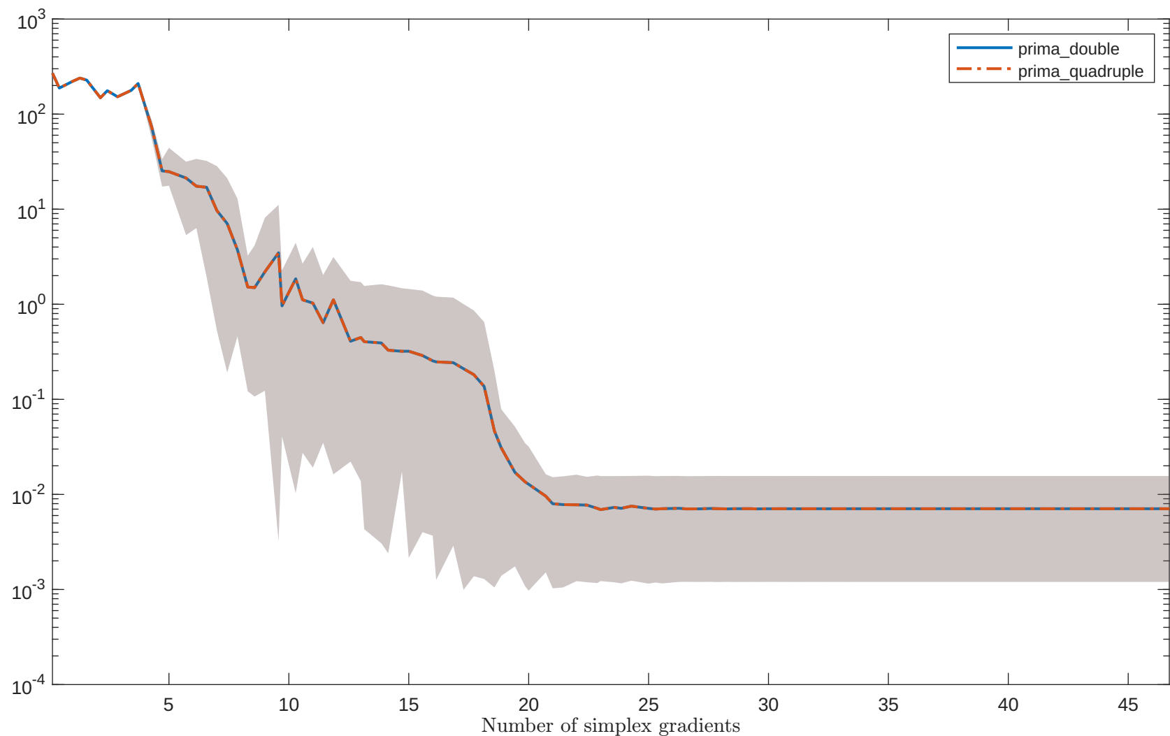
Solving “LANCZOS3LS” with “noisy_0.001_mixed_gaussian” feature
