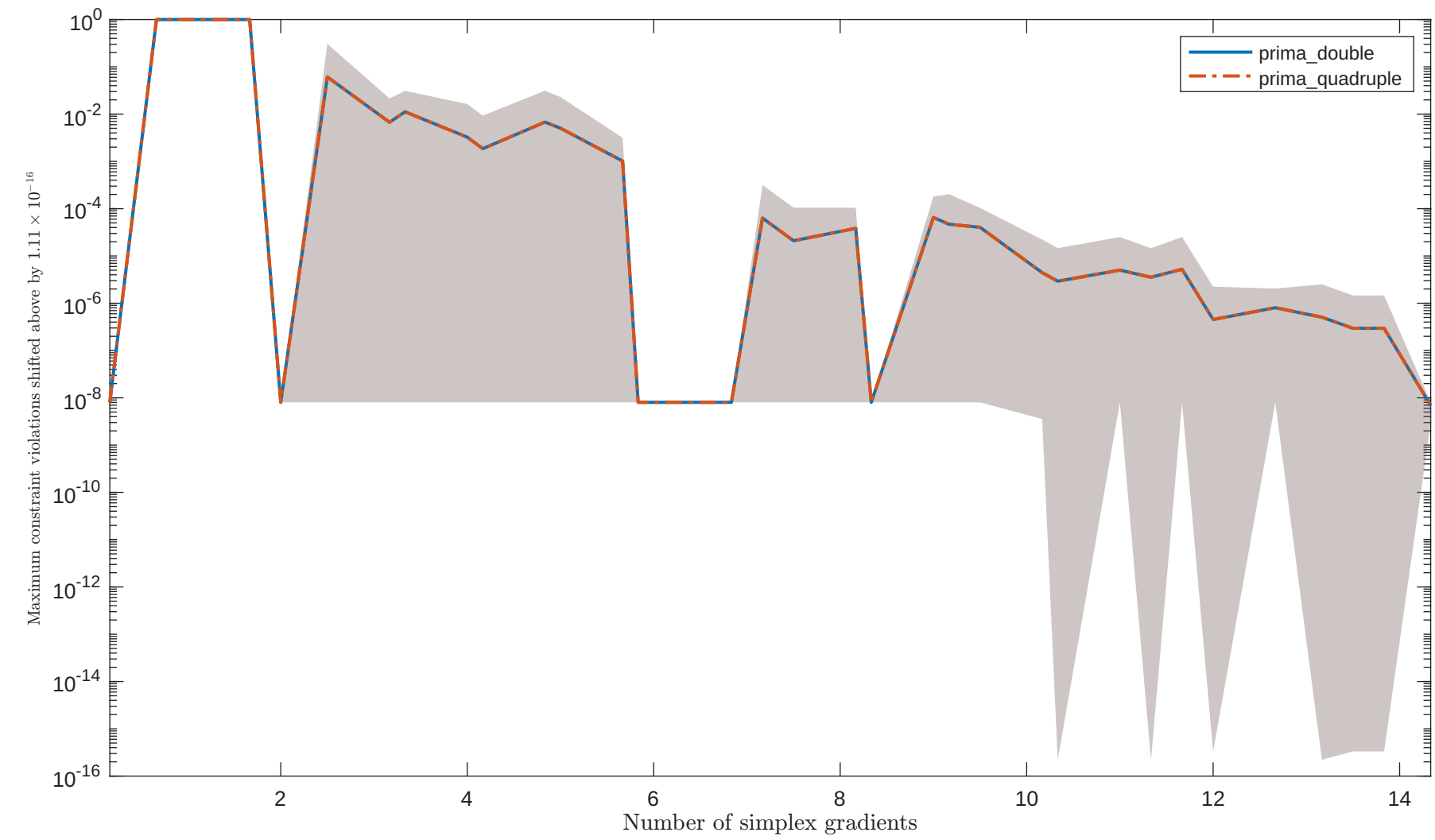
Solving "HS53" with "noisy_0.001_mixed_gaussian" feature
