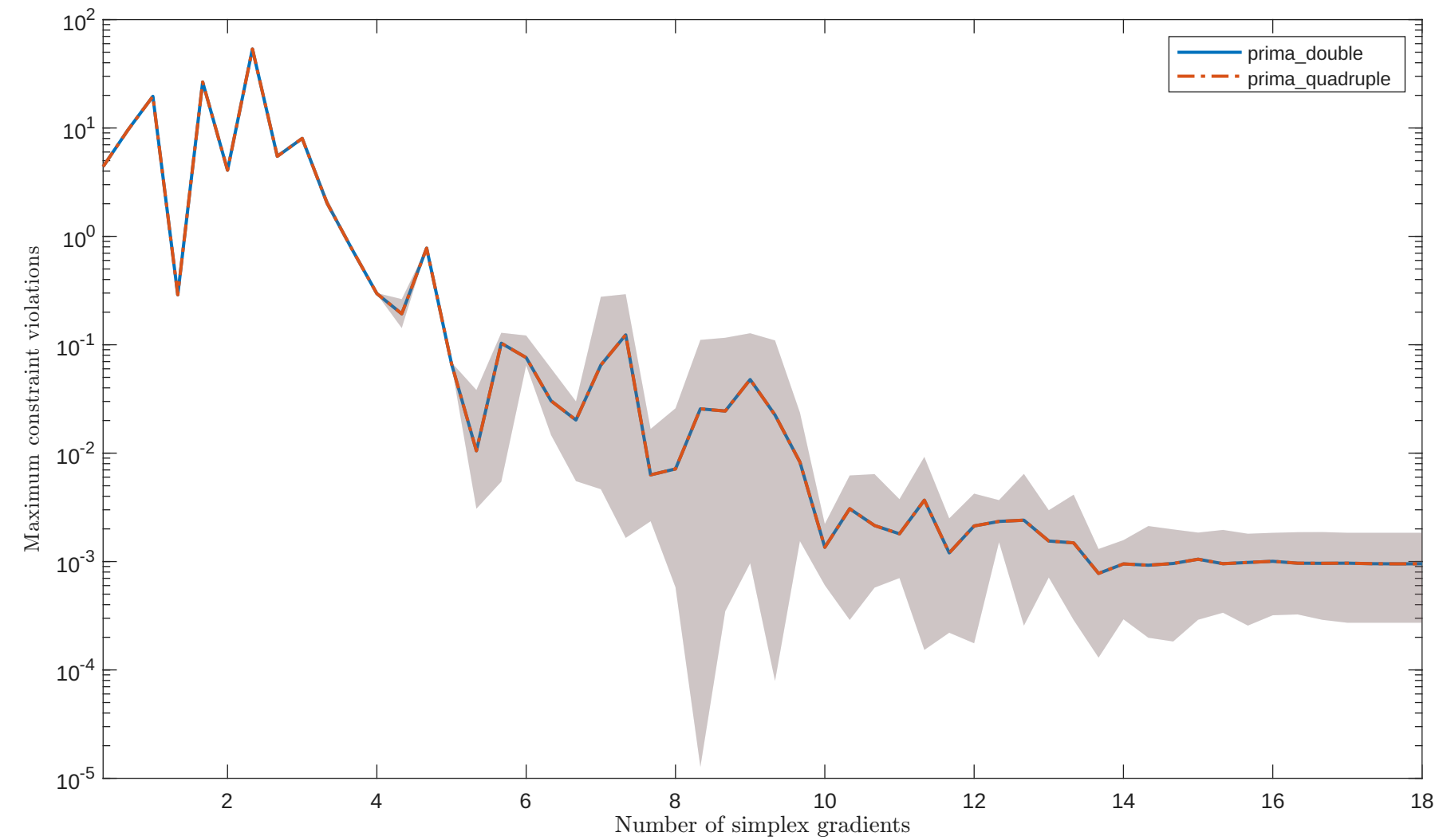
Solving "HS6" with "noisy_0.001_mixed_gaussian" feature
