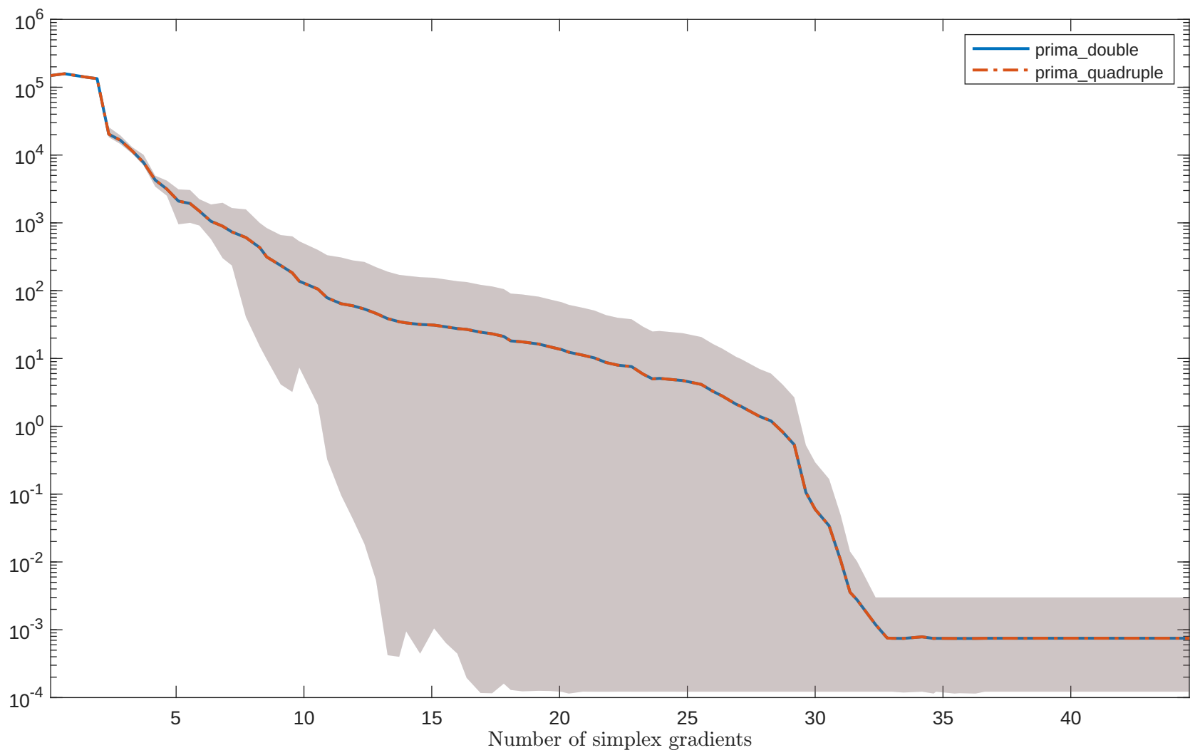
Solving "PENALTY1" with "noisy_0.001_mixed_gaussian" feature
