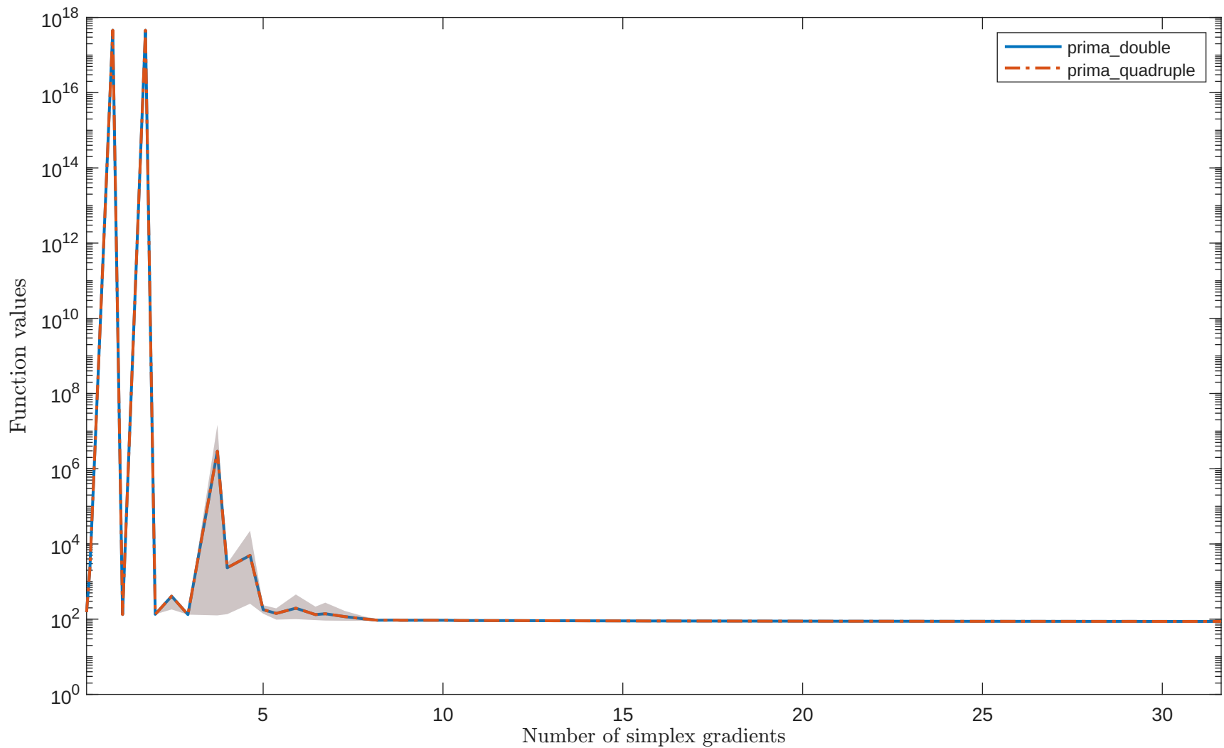
Solving “SBRYBND” with “noisy_0.001_mixed_gaussian” feature
