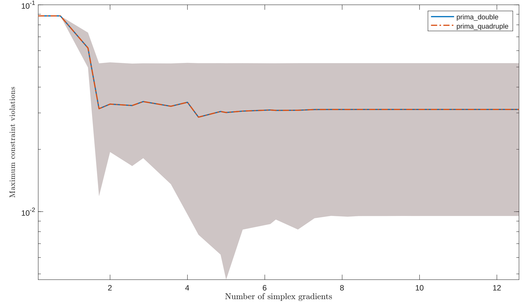
Solving “HS89” with “noisy_0.001_mixed_gaussian” feature
