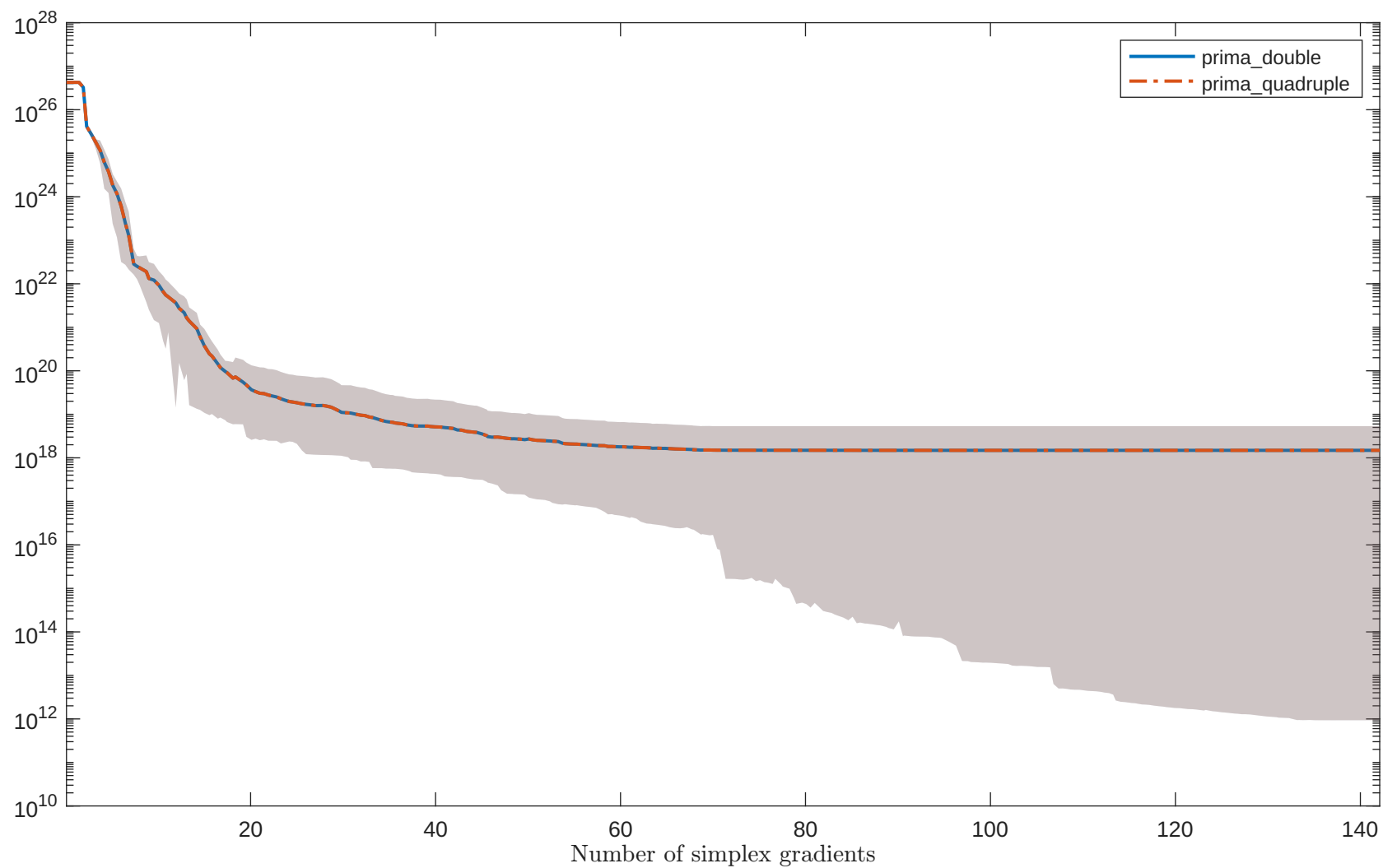
Solving "SCURLY10" with "noisy_0.001_mixed_gaussian" feature
