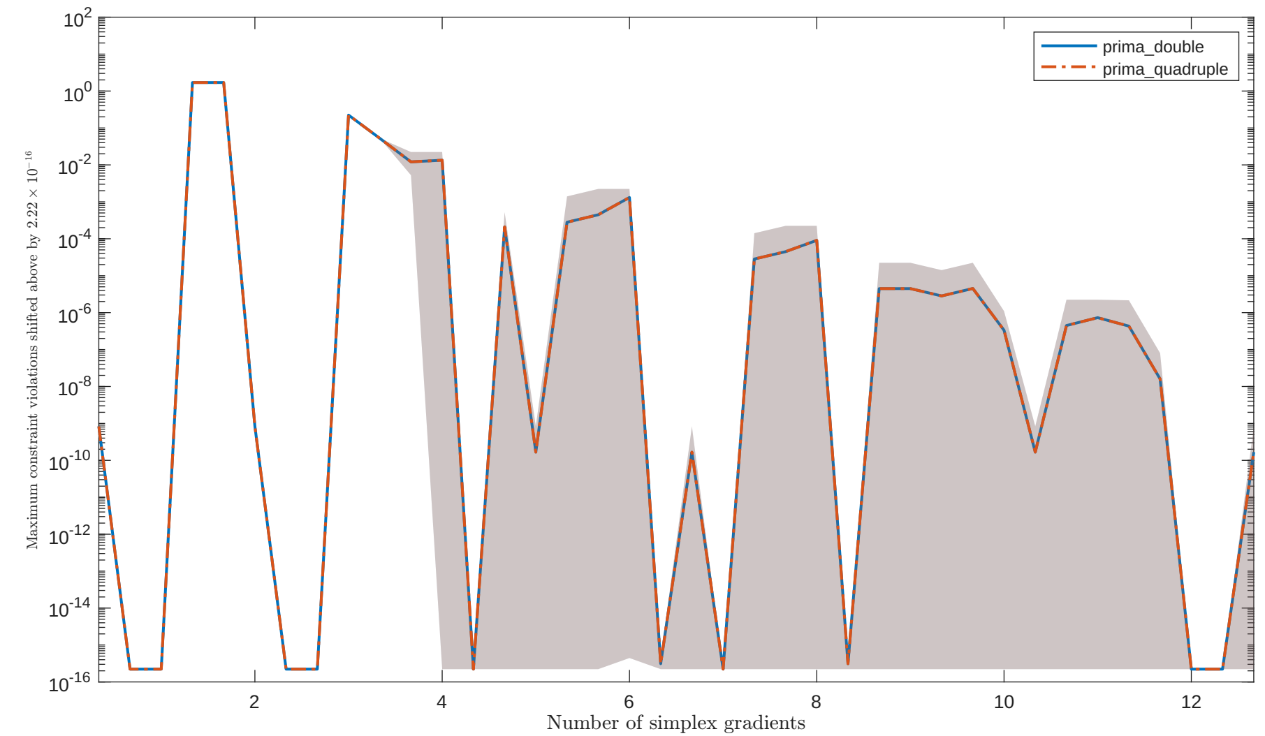
Solving "SIMPLLPB" with "noisy_0.001_mixed.gaussian" feature
