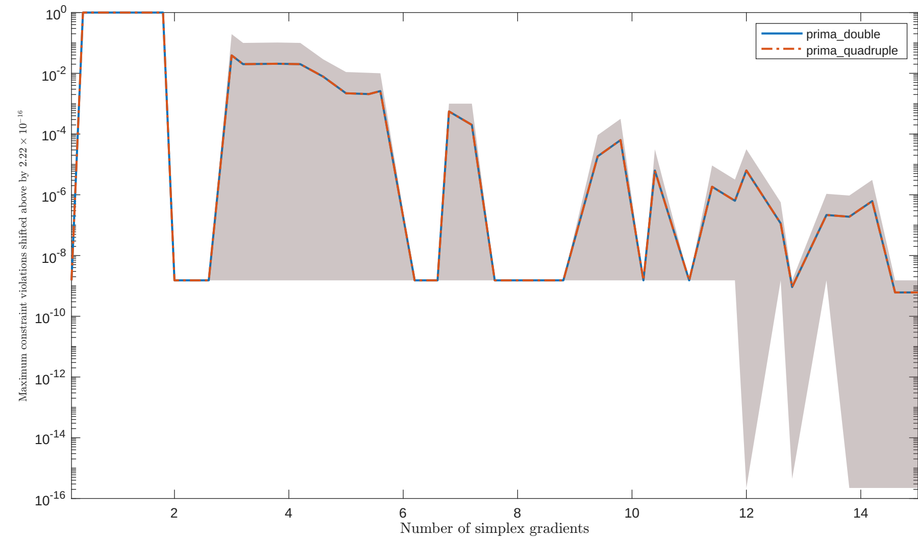
Solving "HS41" with "noisy_0.001_mixed_gaussian" feature
