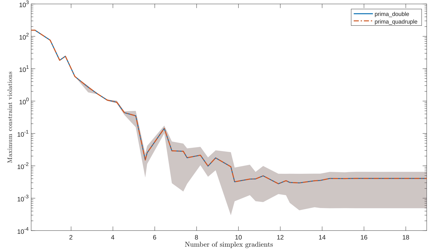
Solving "LUKVLE3" with "noisy_0.001_mixed_gaussian" feature
