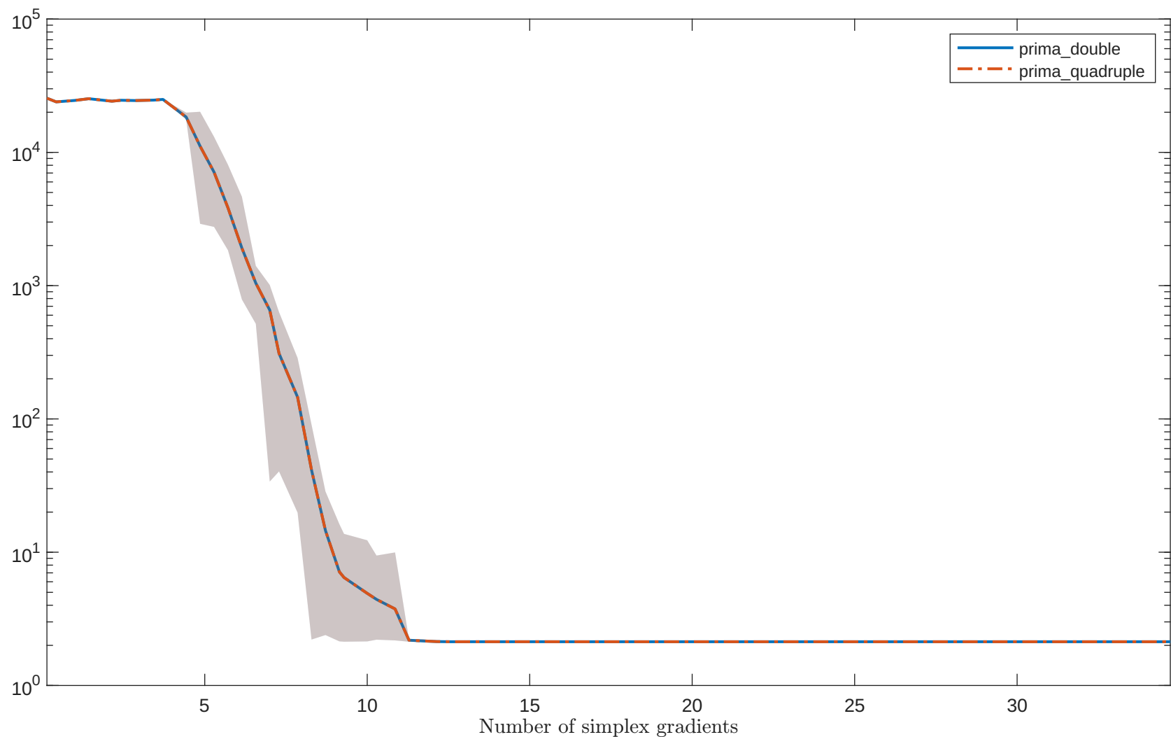
Solving “PALMER5C” with “noisy_0.001_mixed_gaussian” feature
