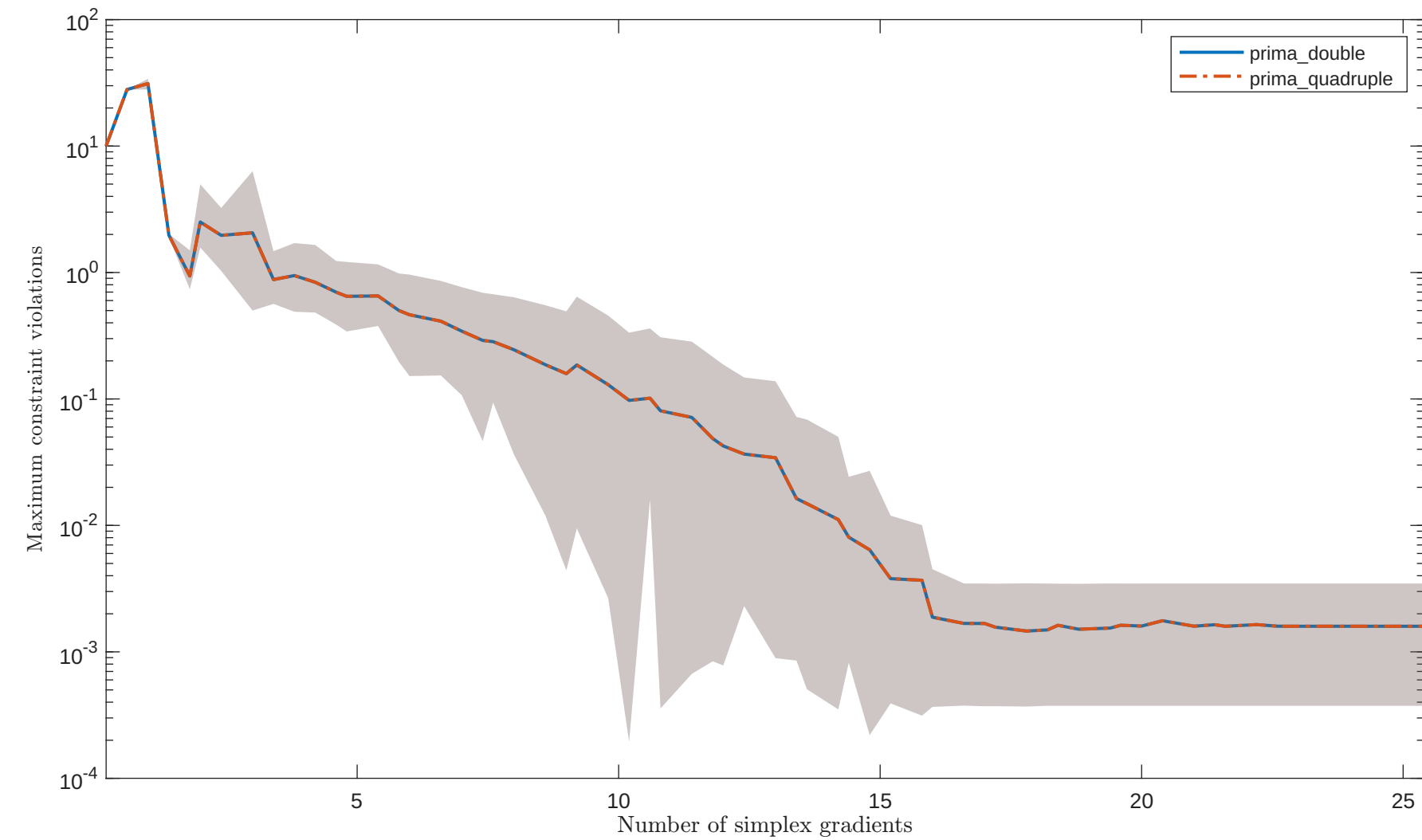
Solving “BT9” with “noisy_0.001_mixed_gaussian” feature
