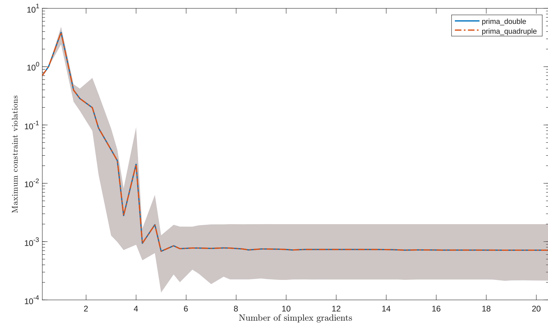
Solving "EIGMAXA" with "noisy_0.001_mixed_gaussian" feature
