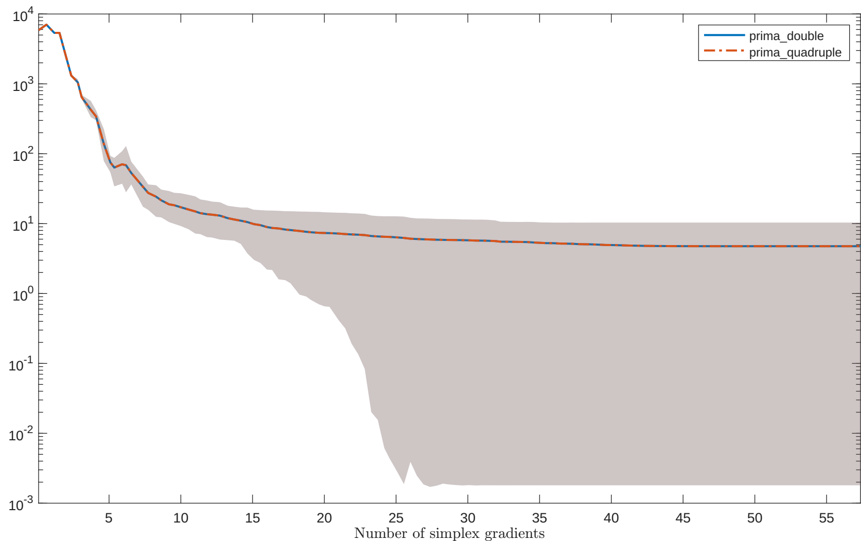
Solving “LIARWHD” with “noisy_0.001_mixed_gaussian” feature
