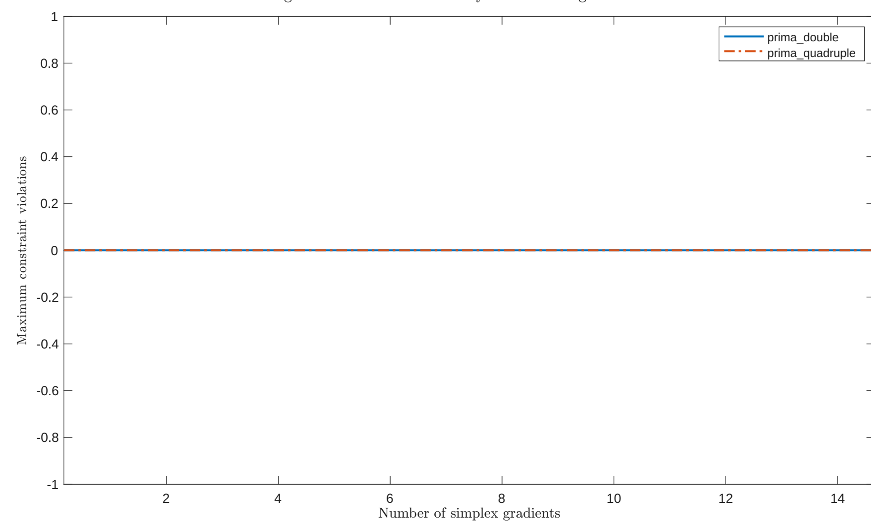
Solving “DEVGLA2B” with “noisy_0.001_mixed_gaussian” feature
