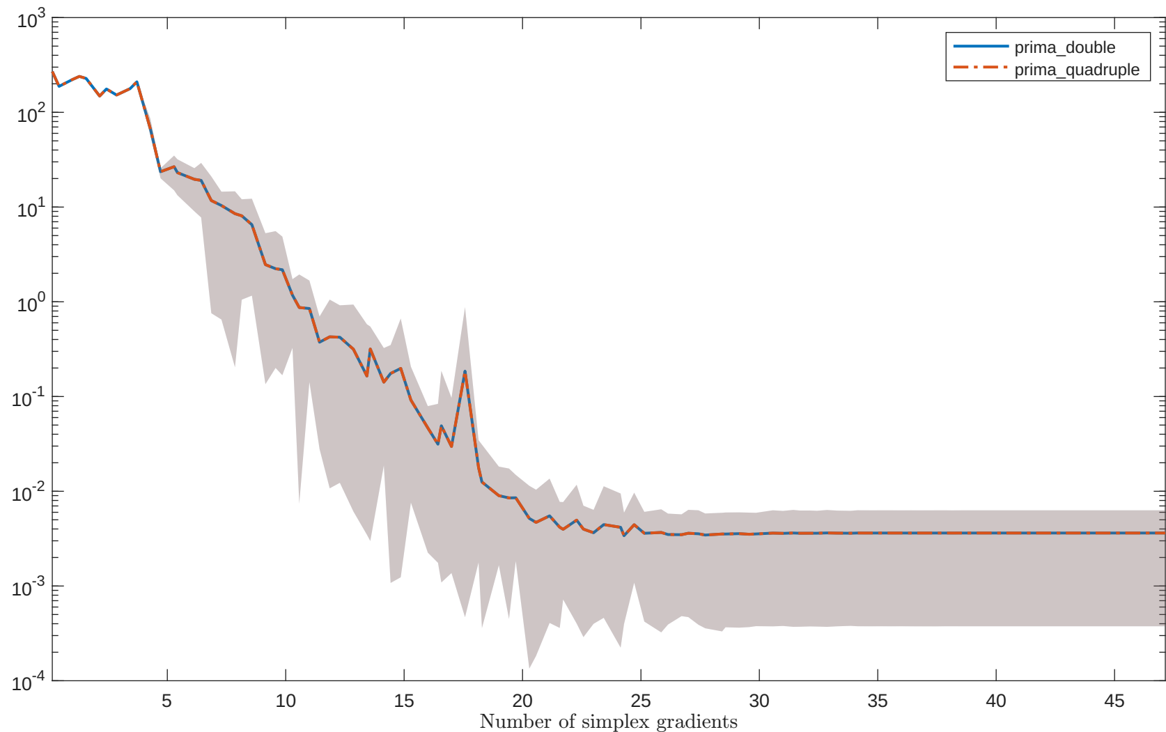
Solving “LANCZOS2LS” with “noisy_0.001_mixed_gaussian” feature
