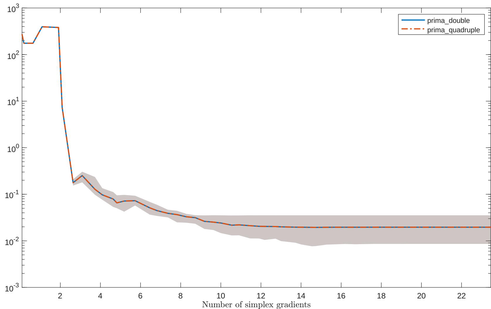
Solving “BROWNAL” with “noisy_0.001_mixed_gaussian” feature
