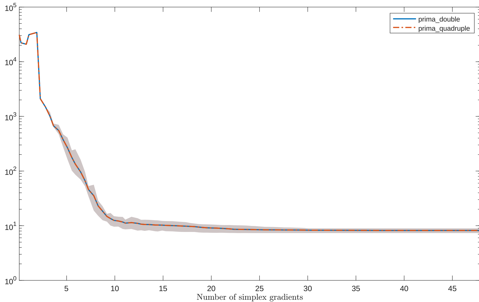
Solving “ERRINRSM” with “noisy_0.001_mixed_gaussian” feature
