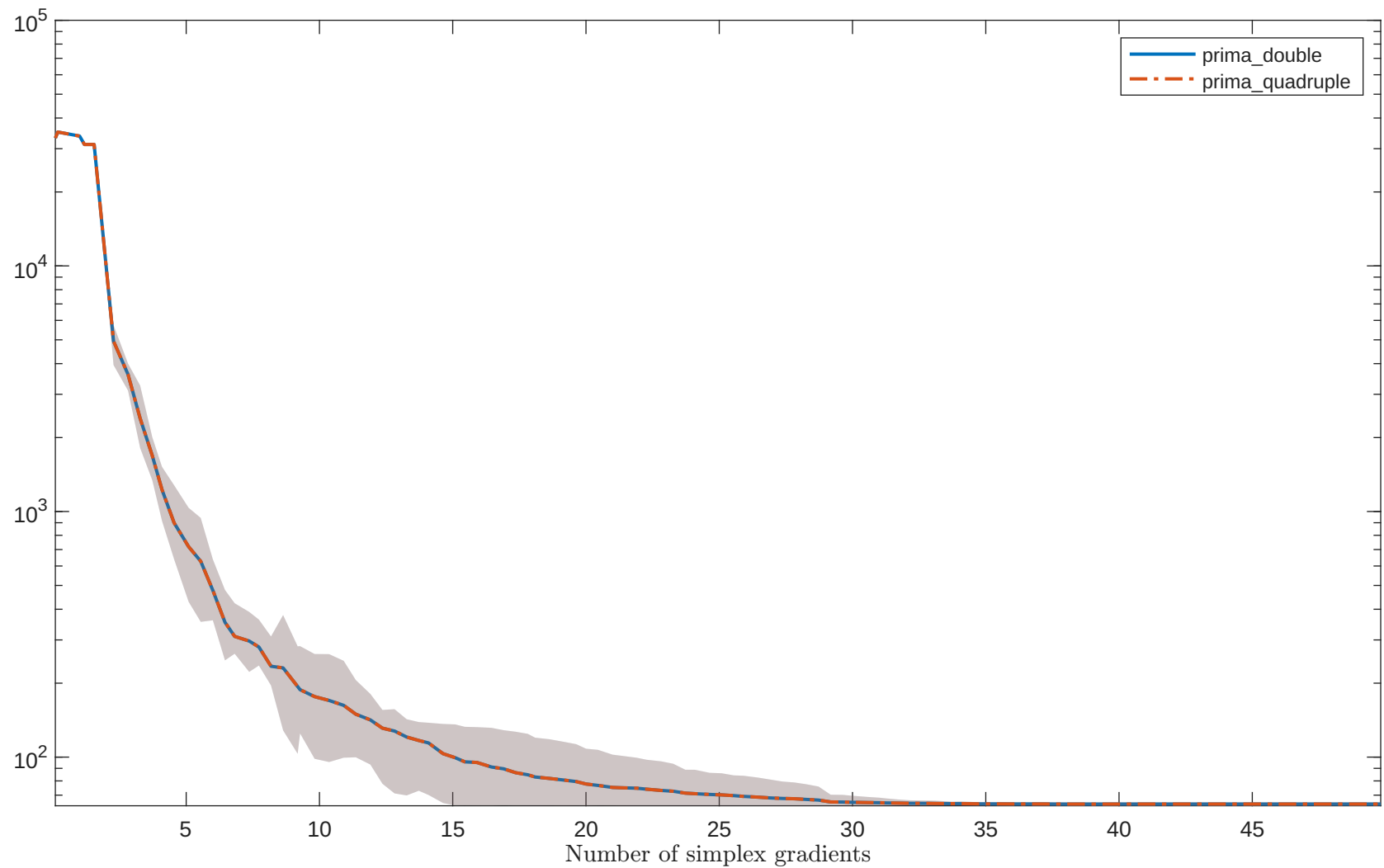
Solving “EDENSCH” with “noisy_0.001_mixed_gaussian” feature
