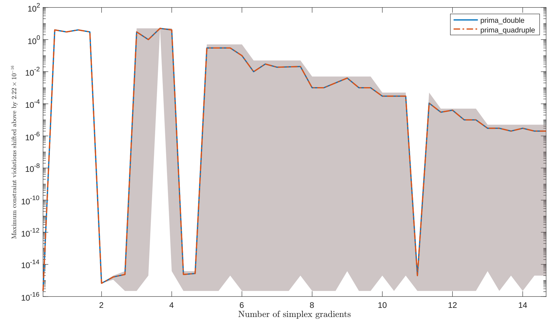
Solving "HS9" with "noisy_0.001_mixed_gaussian" feature
