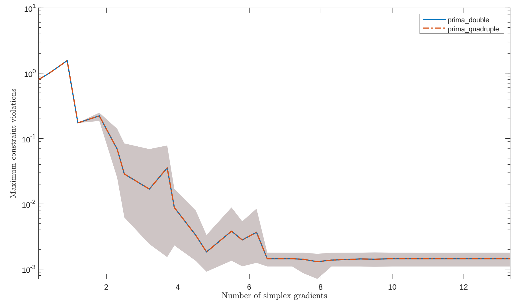
Solving "HS107" with "noisy_0.001_mixed_gaussian" feature
