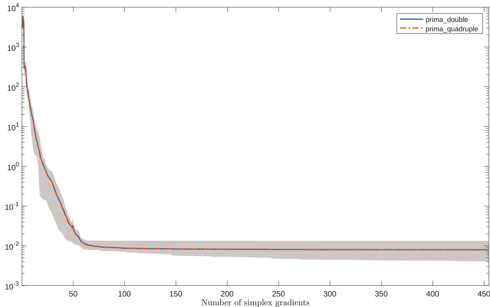
Solving “EXTROSNB” with “noisy_0.001_mixed-gaussian” feature
