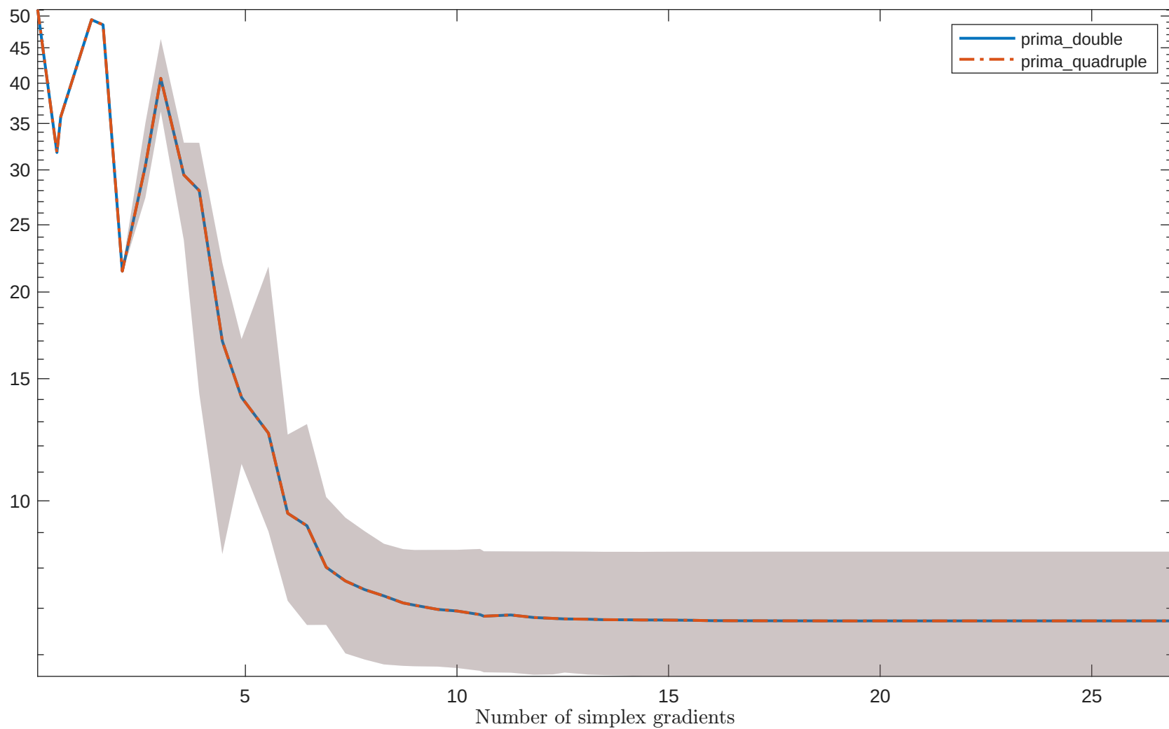
Solving "TRIGON2" with "noisy_0.001_mixed_gaussian" feature
