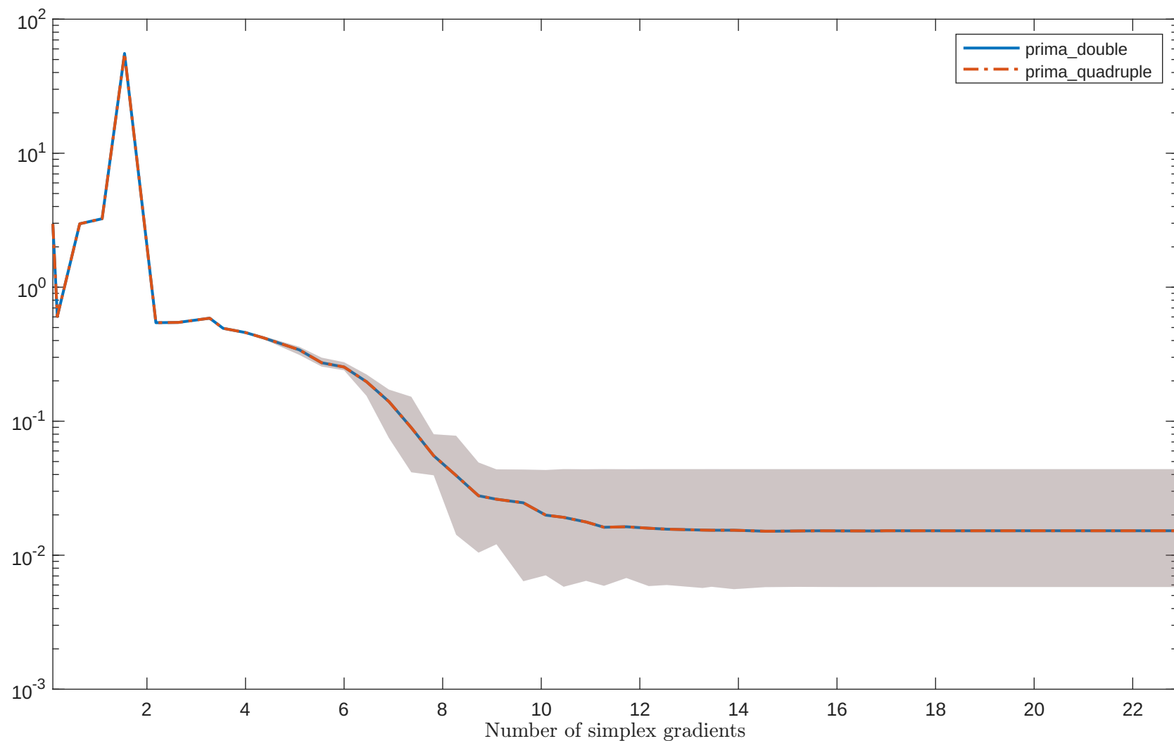
Solving "ARGTRIGLS" with "noisy_0.001_mixed_gaussian" feature
