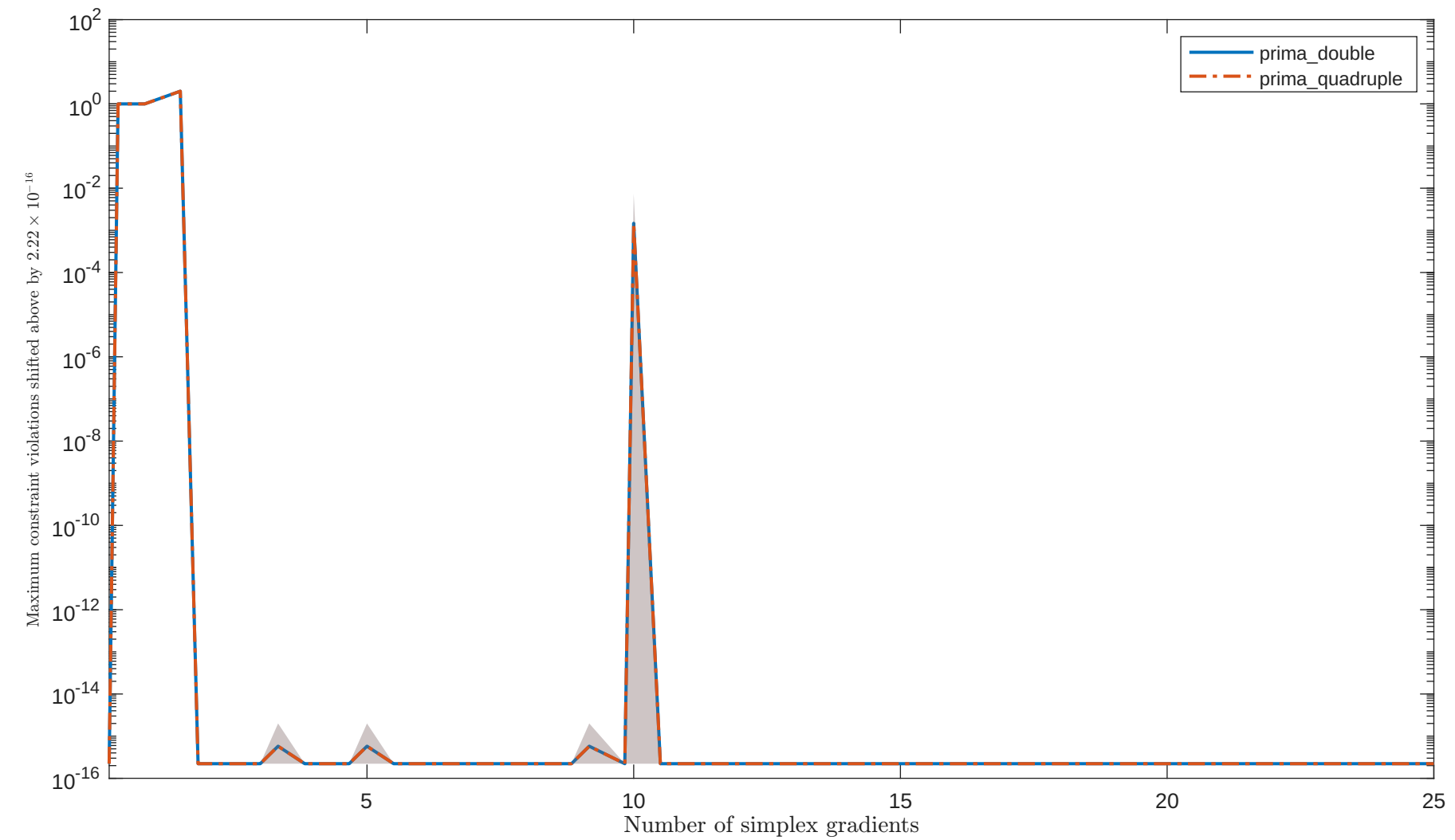
Solving “HS268” with “noisy_0.001_mixed_gaussian” feature
