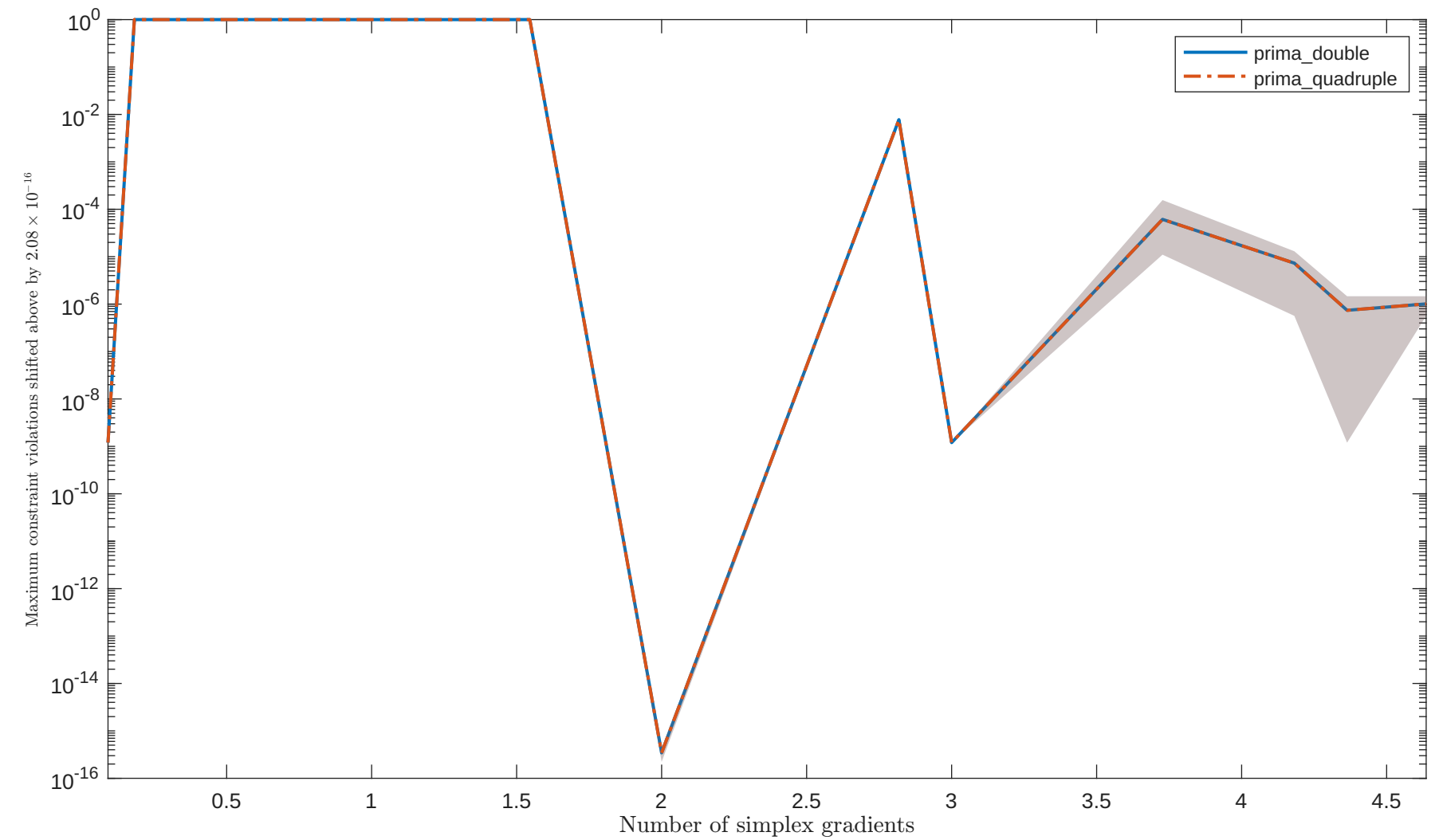
Solving “PORTSNQP” with “noisy_0.001_mixed-gaussian” feature
