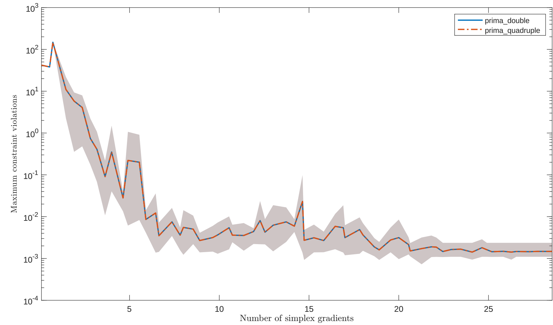
Solving “LUKVL14” with “noisy_0.001_mixed_gaussian” feature
