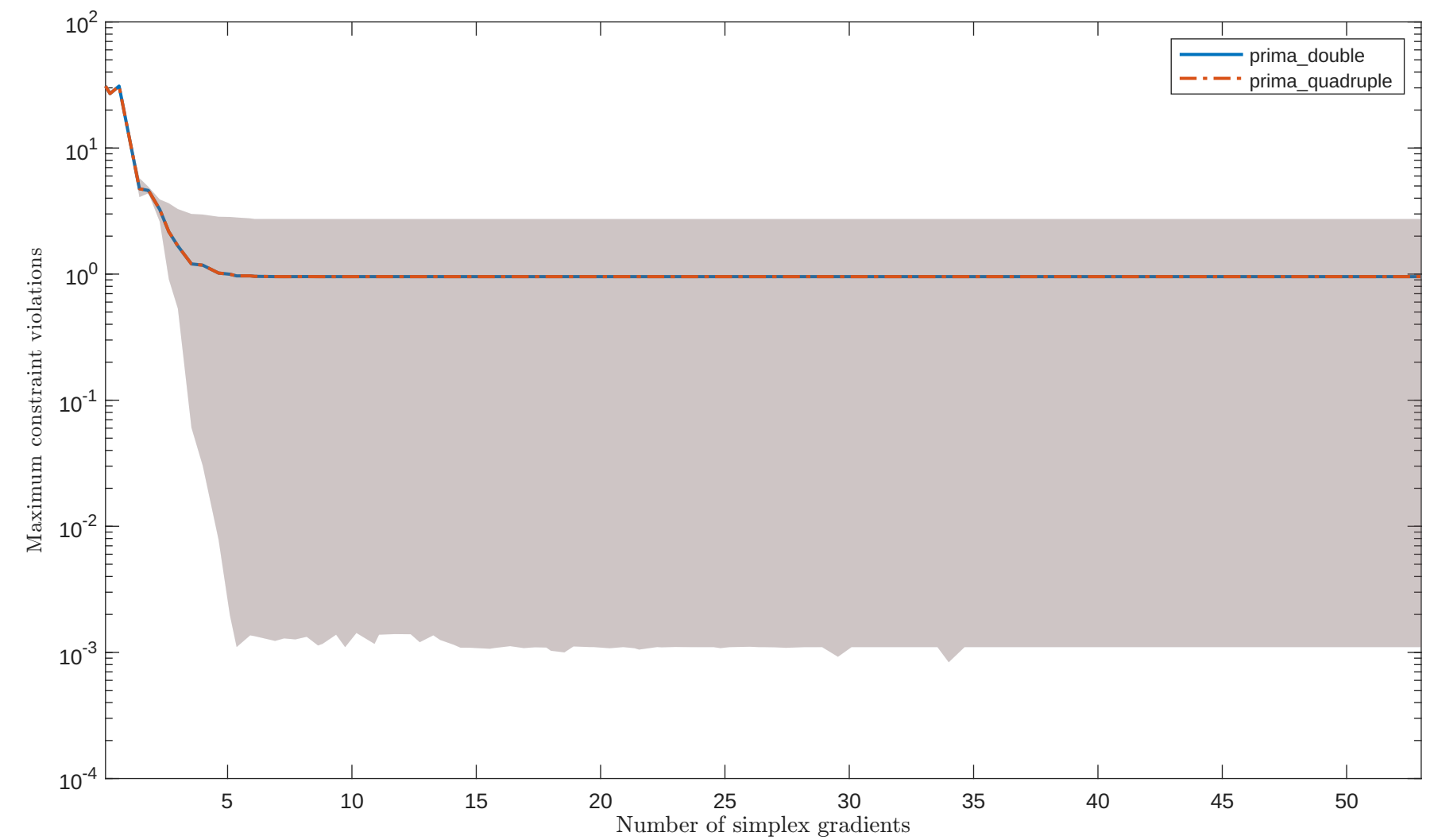
Solving “LUKVLE9” with “noisy_0.001_mixed_gaussian” feature
