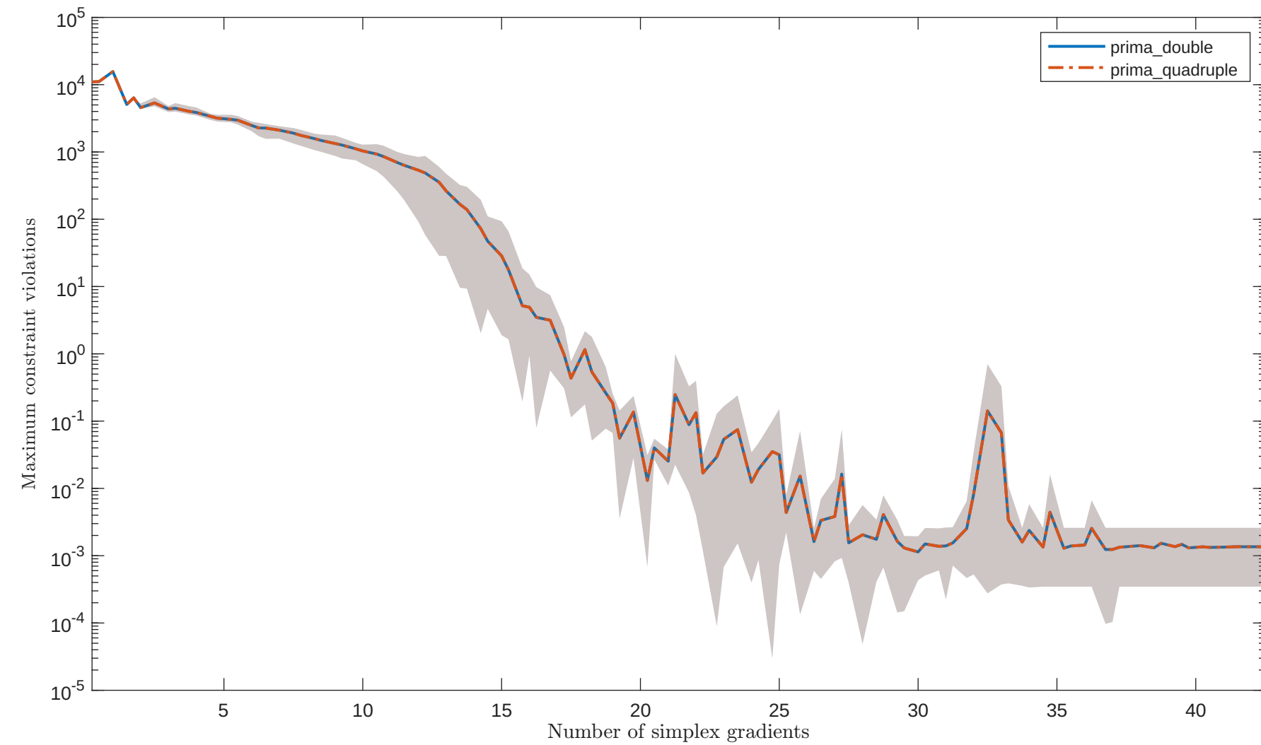
Solving "BT2" with "noisy_0.001_mixed_gaussian" feature
