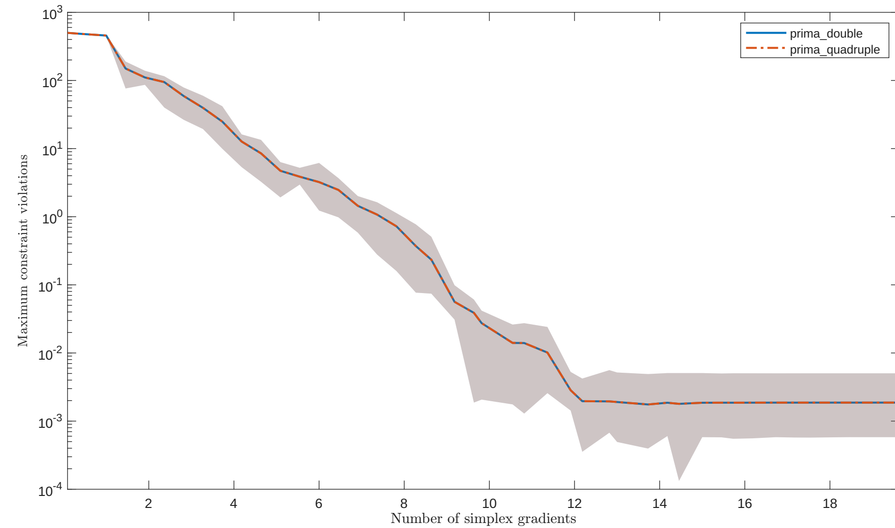
Solving "GILBERT" with "noisy_0.001_mixed-gaussian" feature
