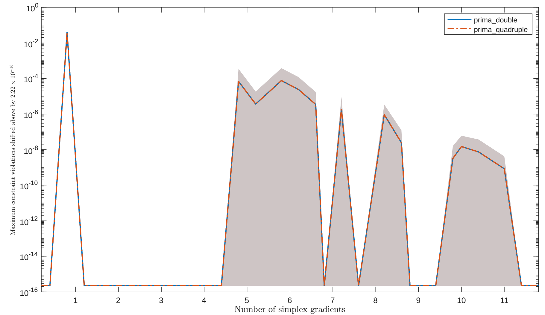
Solving “HS70” with “noisy_0.001_mixed_gaussian” feature
