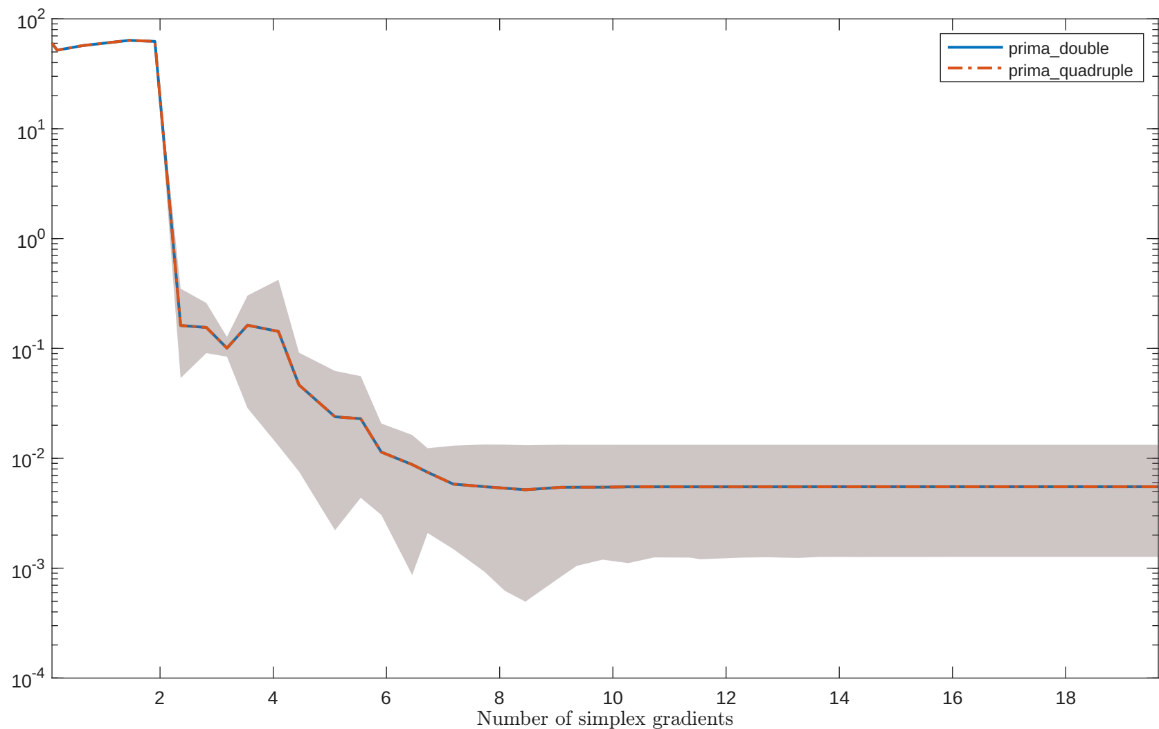
Solving "HILBERTA" with "noisy_0.001_mixed_gaussian" feature
