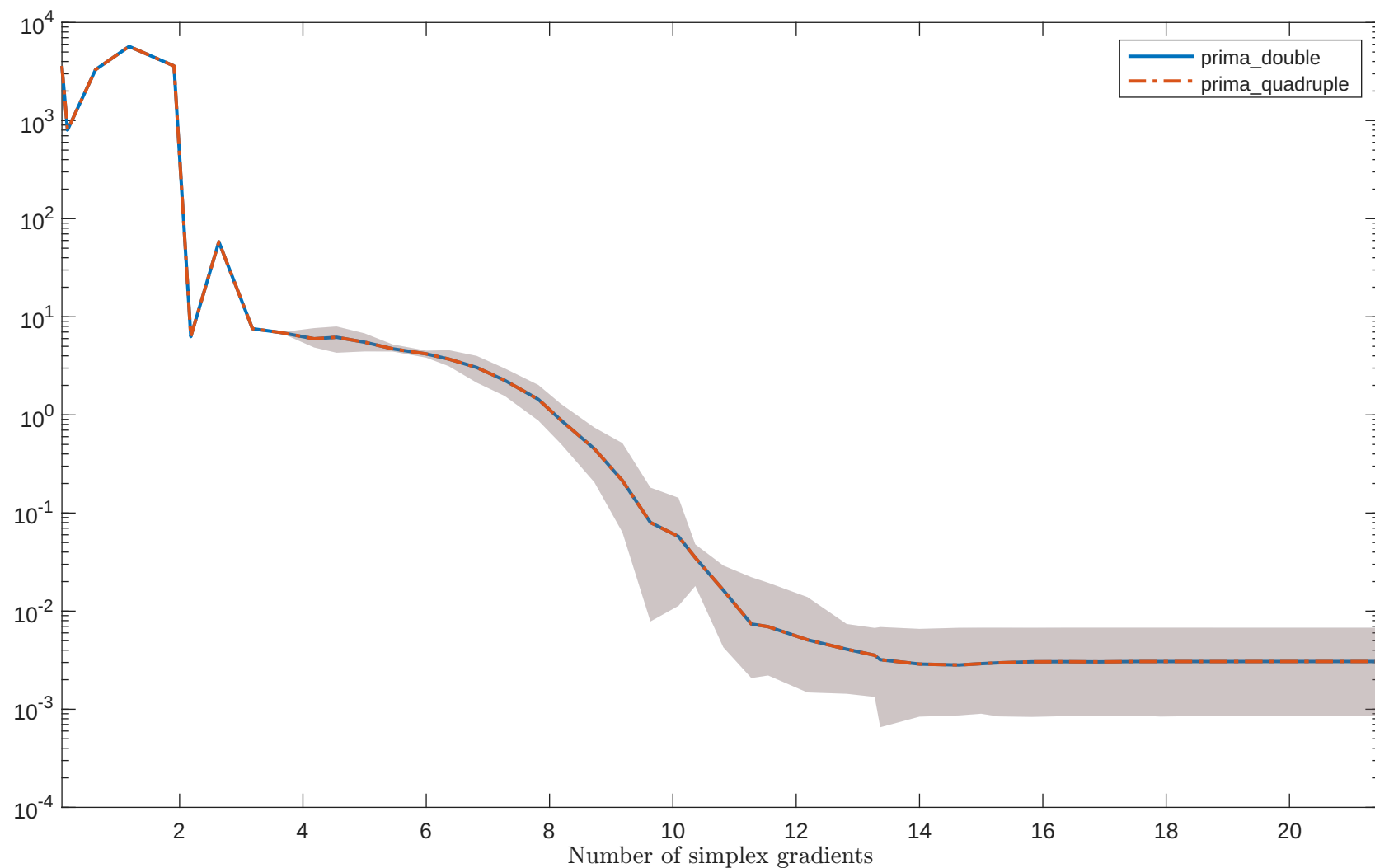
Solving “NONDIA” with “noisy_0.001_mixed_gaussian” feature
