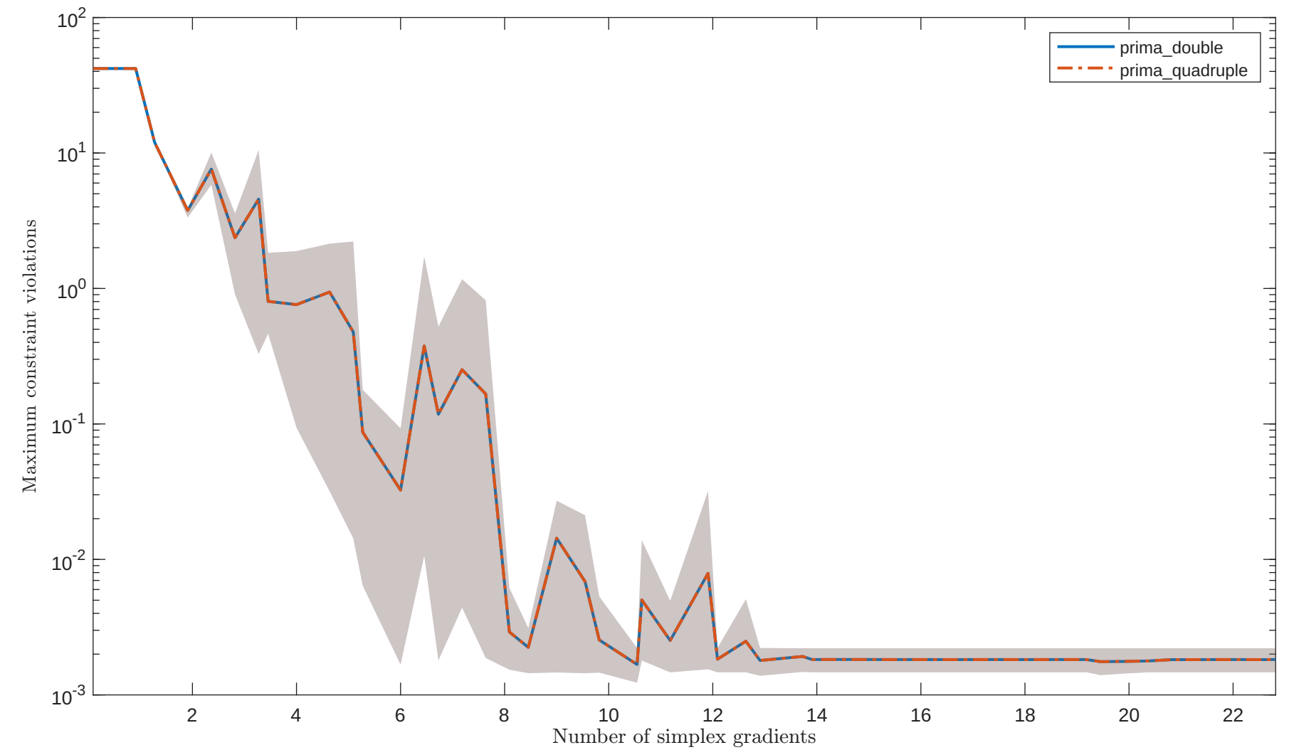
Solving "LUKVLE4C" with "noisy_0.001_mixed_gaussian" feature
