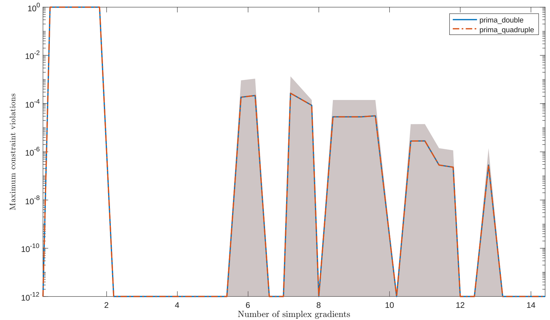
Solving "LIN" with "noisy_0.001_mixed_gaussian" feature
