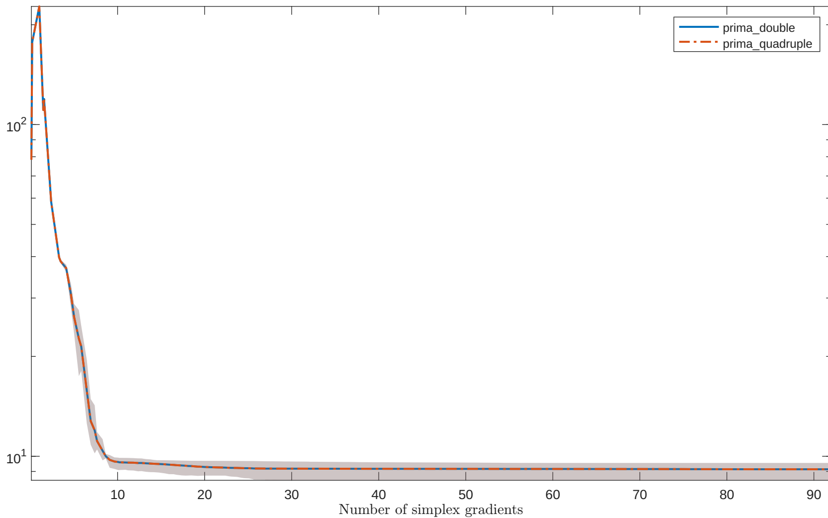
Solving “GENROSE” with “noisy_0.001_mixed_gaussian” feature
