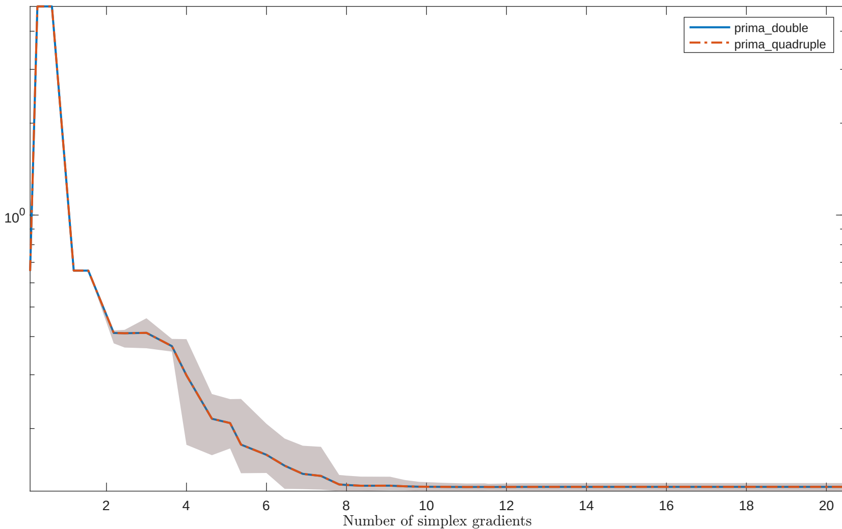
Solving “SINQUAD2” with “noisy_0.001_mixed_gaussian” feature
