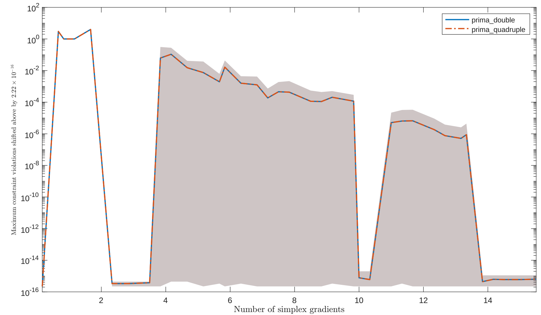
Solving “HS86” with “noisy_0.001_mixed.gaussian” feature
