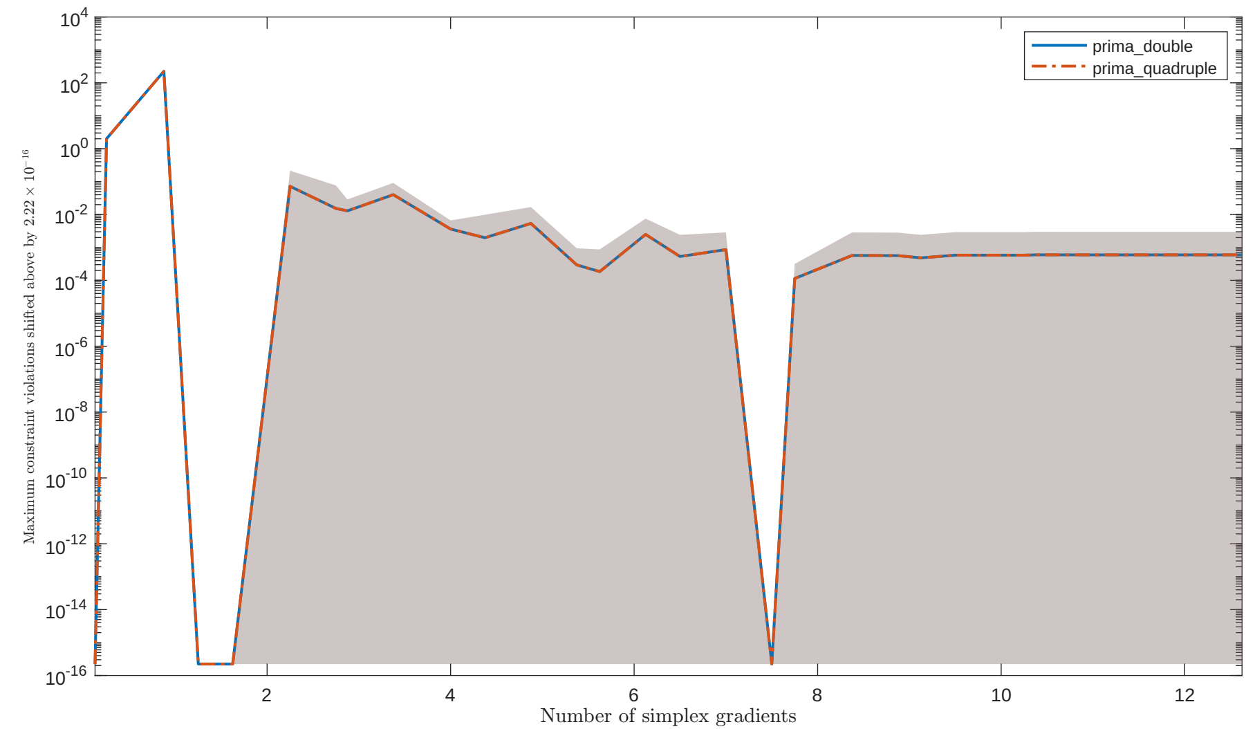
Solving “HS100” with “noisy_0.001_mixed_gaussian” feature
