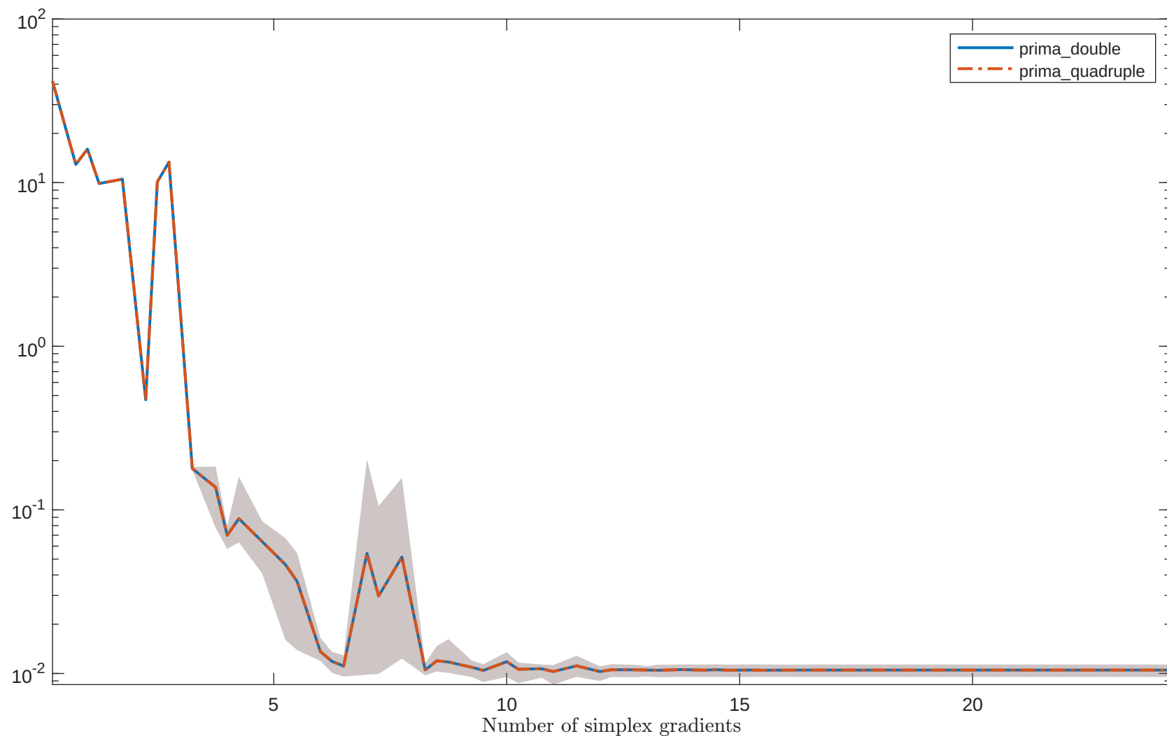
Solving “BARD” with “noisy_0.001_mixed_gaussian” feature
