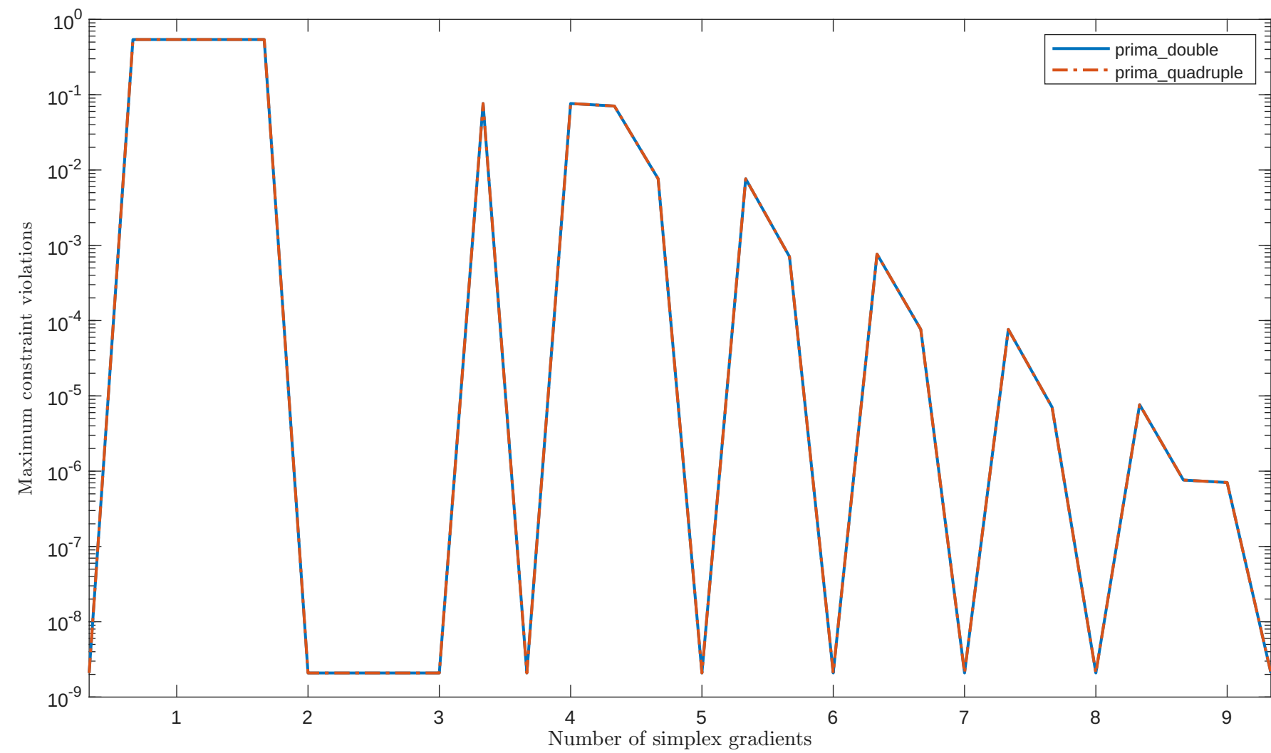
Solving “ALSTAME” with “plain” feature
