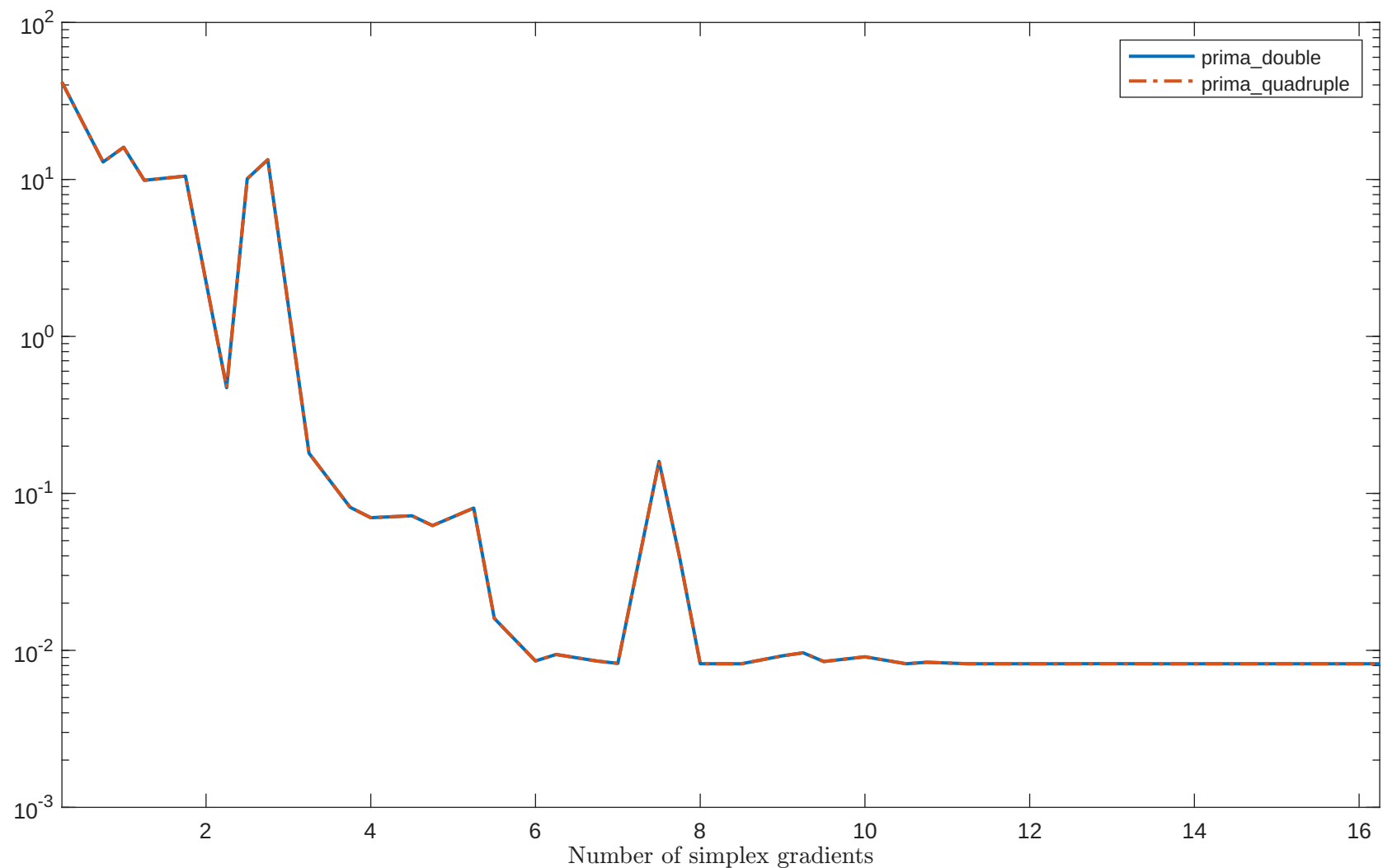
Solving “BARD” with “plain” feature
