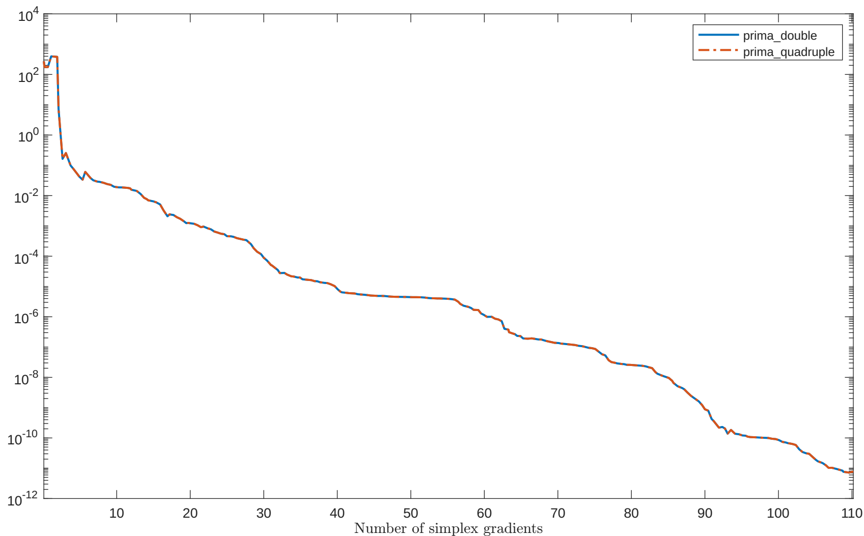
Solving "BROWNAL" with "plain" feature
