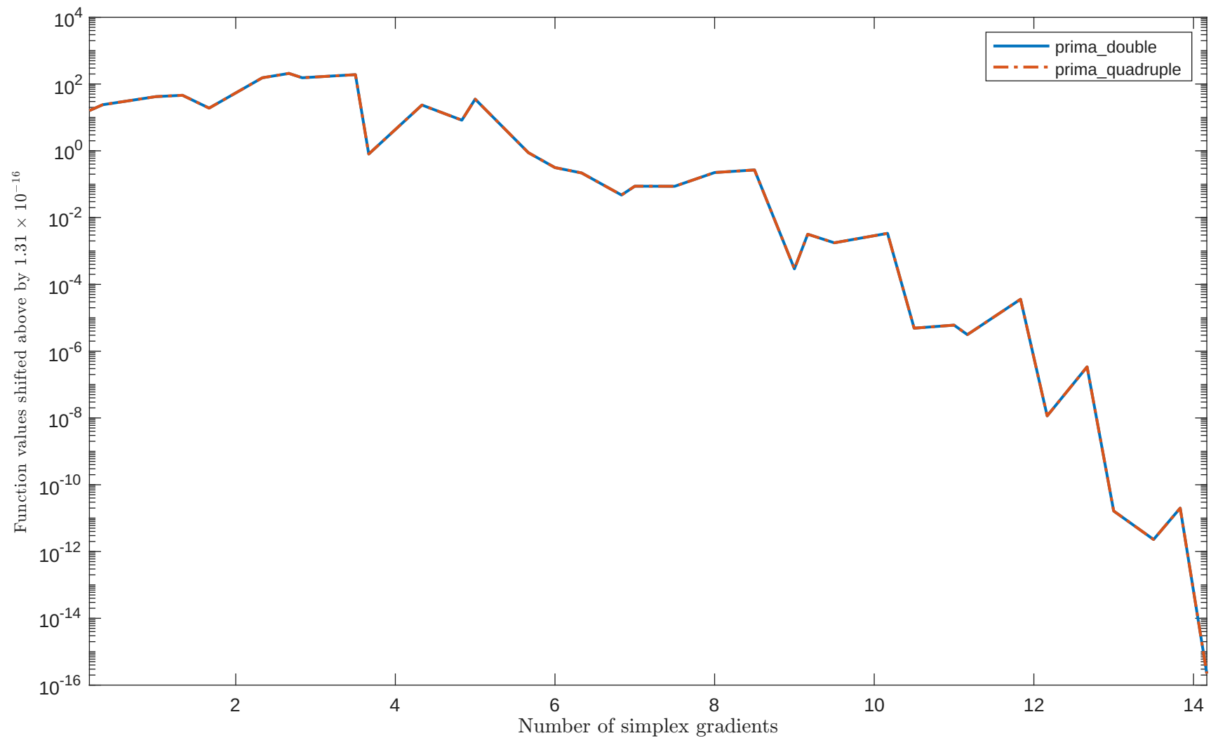
Solving "BROYDN3DLS" with "plain" feature
