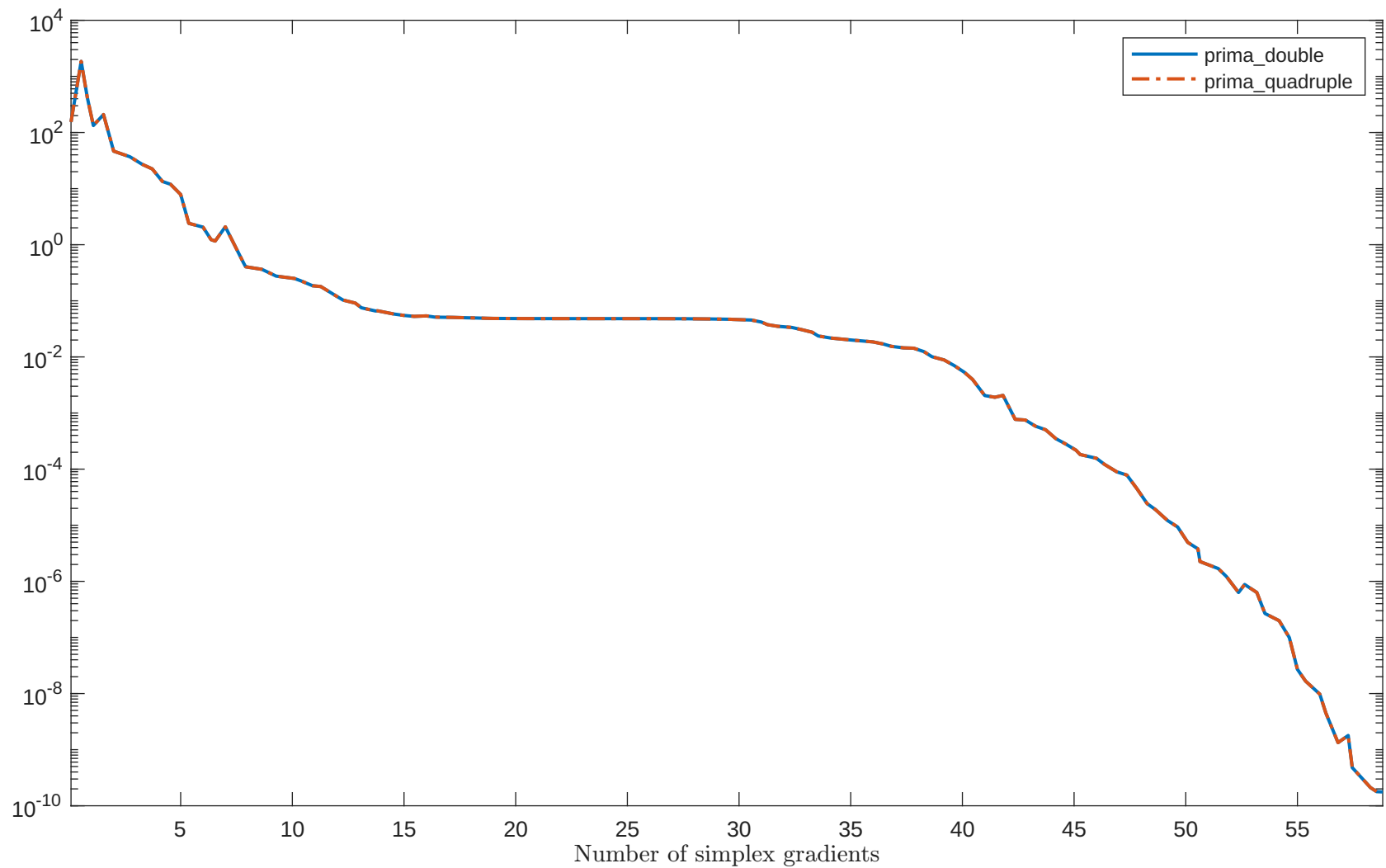
Solving “BRYBND” with “plain” feature
