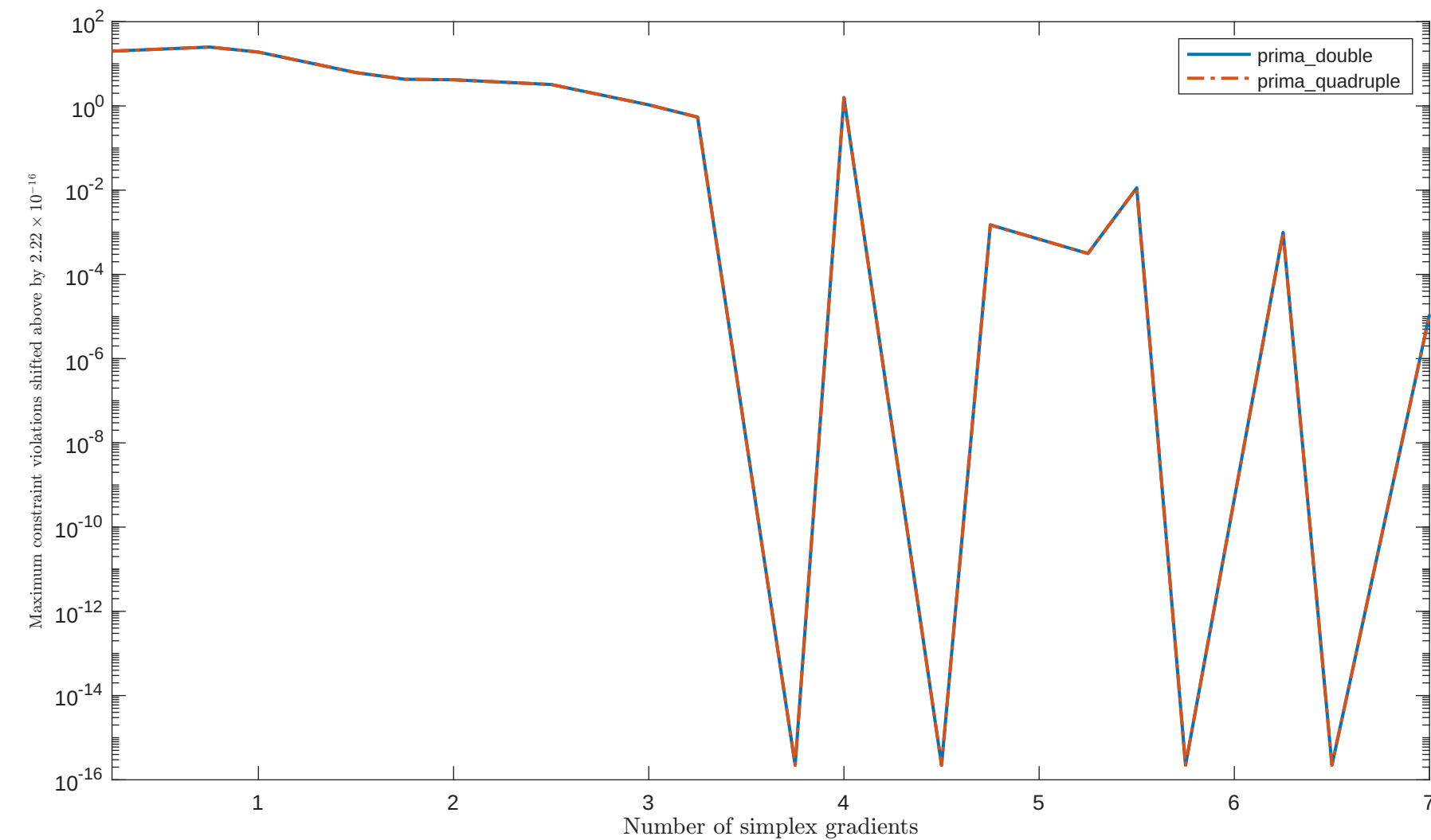
Solving "CHACONN2" with "plain" feature
