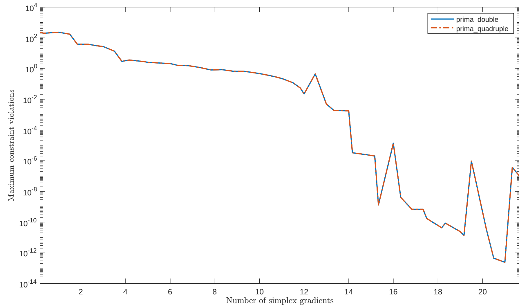
Solving "CSFI2" with "plain" feature
