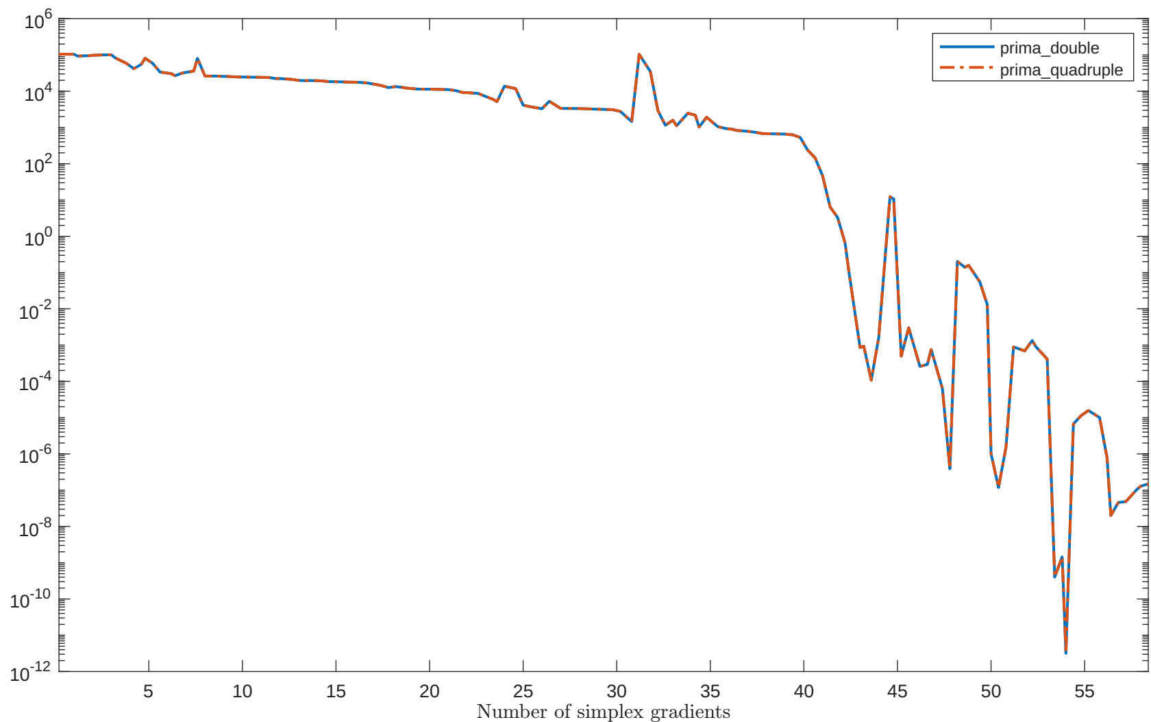
Solving "DEVGLA1" with "plain" feature
