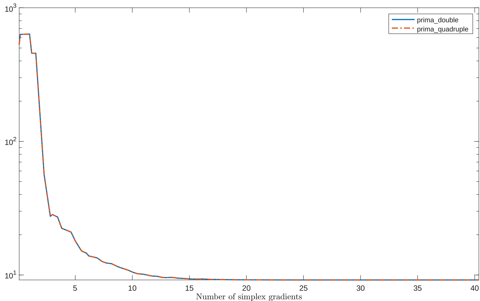
Solving “ENGVAL1” with “plain” feature
