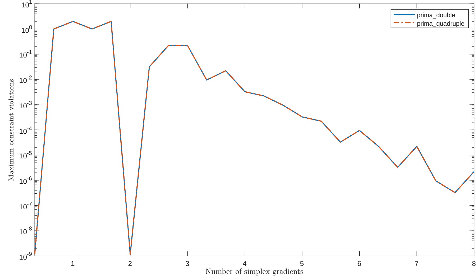
Solving "EXTRASIM" with "plain" feature
