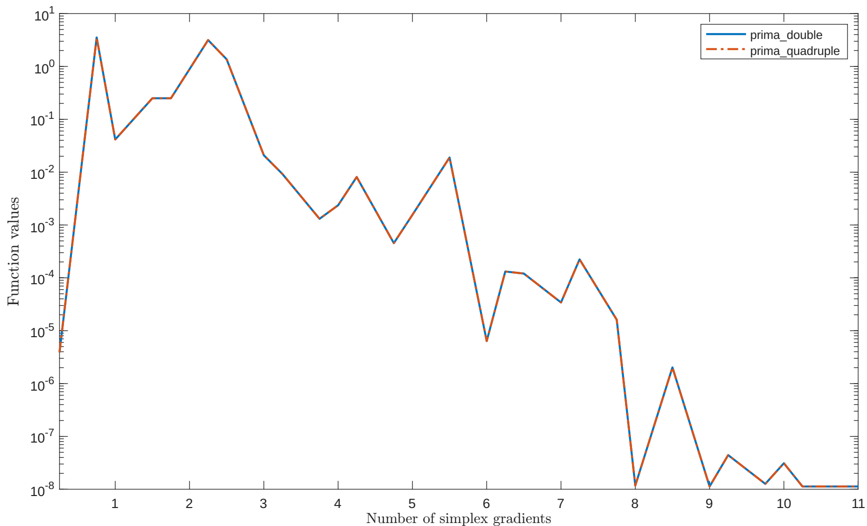
Solving "GAUSSIAN" with "plain" feature
