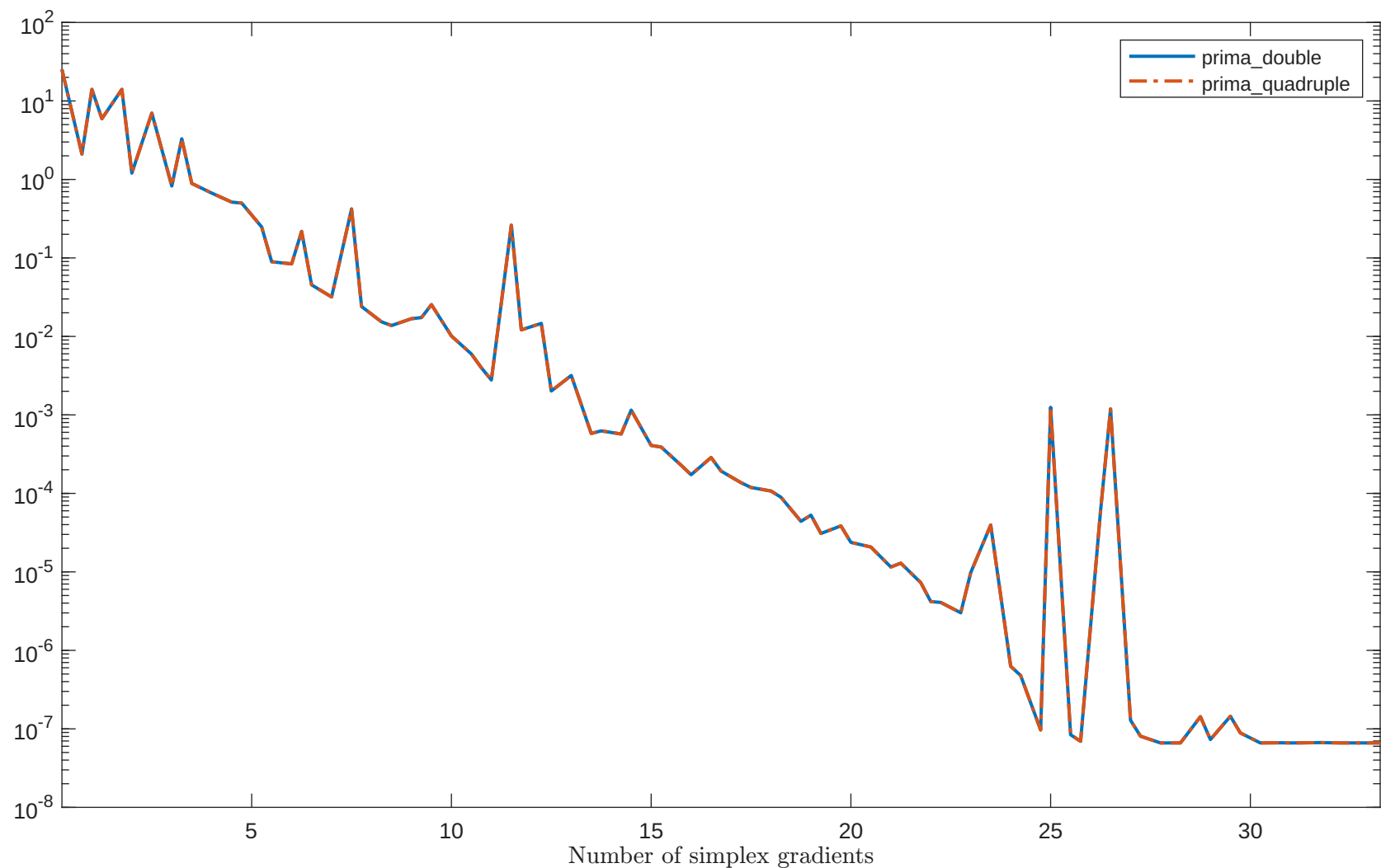
Solving "HATFLDD" with "plain" feature
