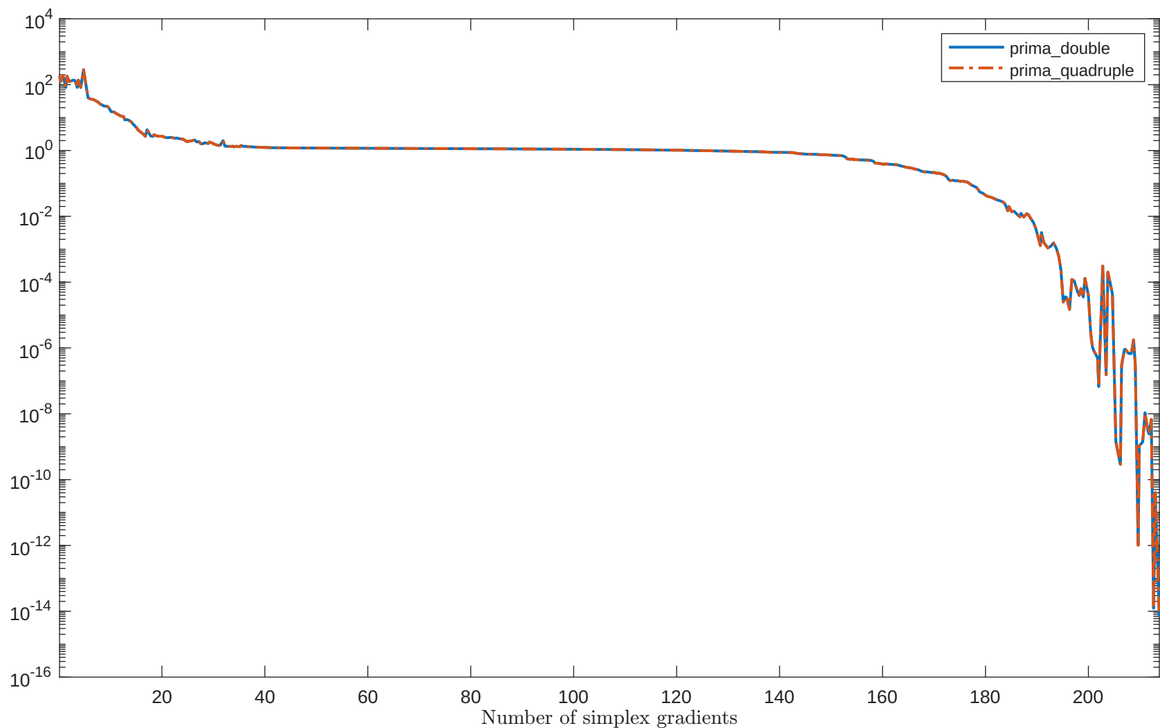
Solving "HEART8LS" with "plain" feature
