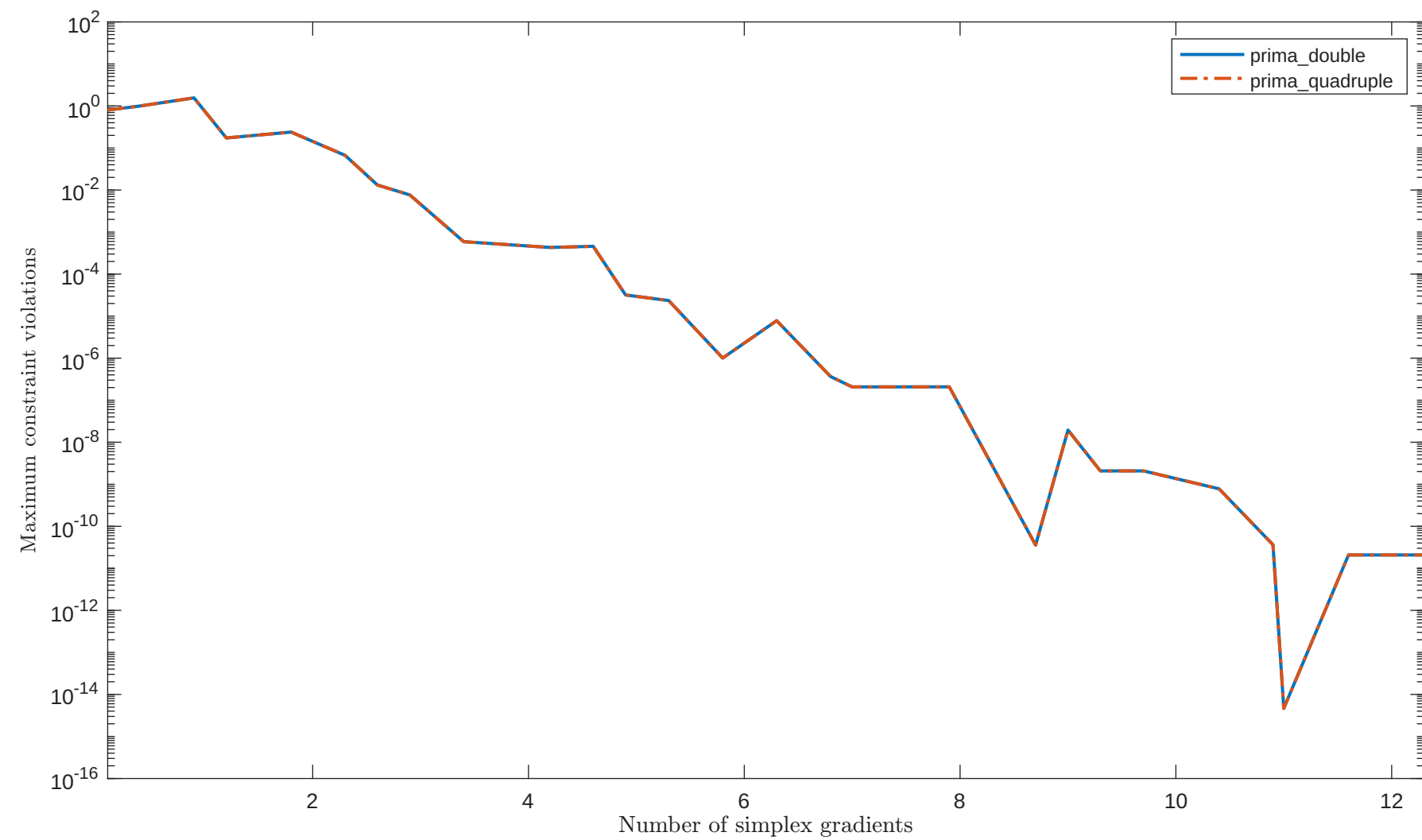
Solving "HS107" with "plain" feature
