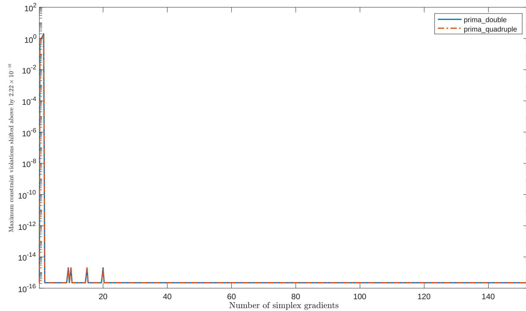
Solving "HS268" with "plain" feature
