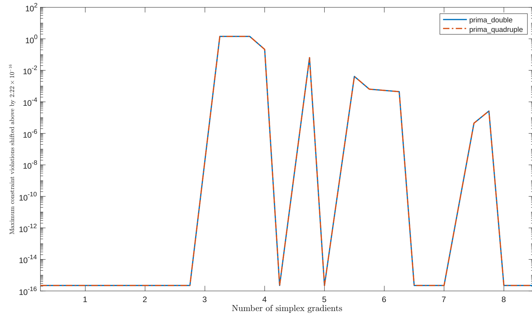
Solving "HS36" with "plain" feature
