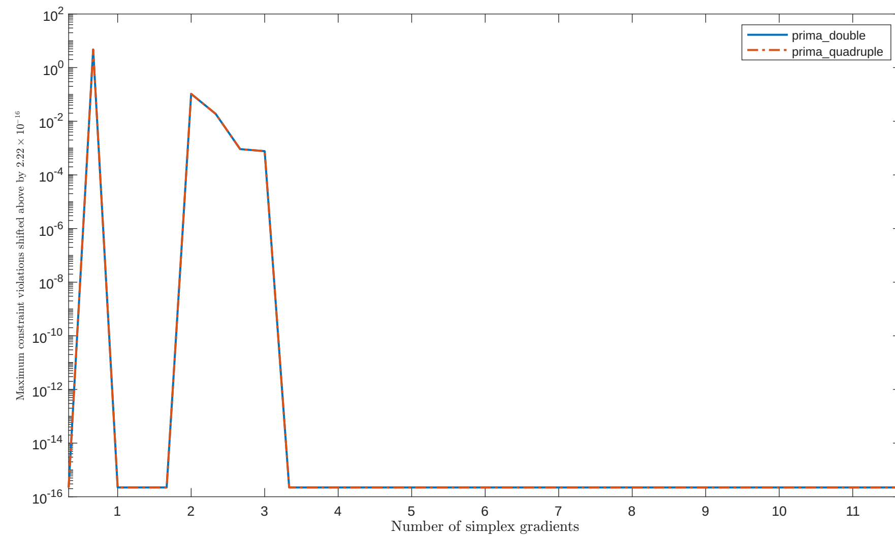
Solving "HS57" with "plain" feature
