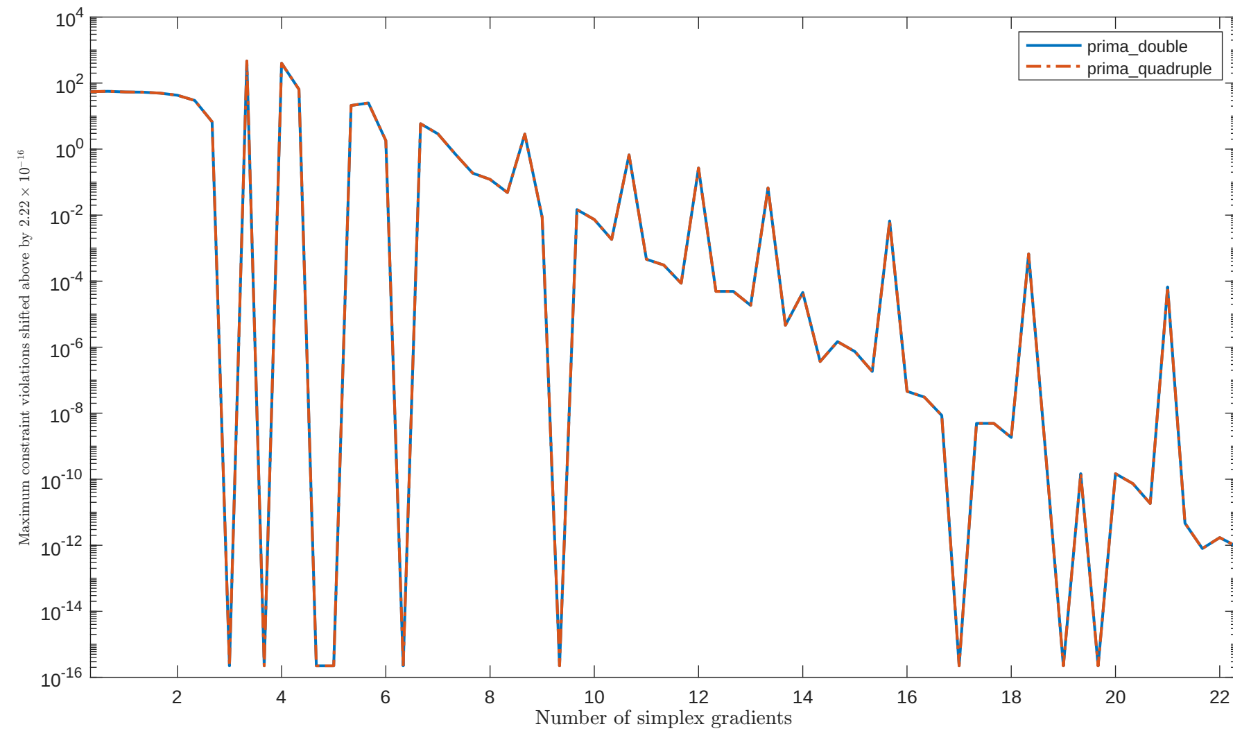
Solving "HS59" with "plain" feature
