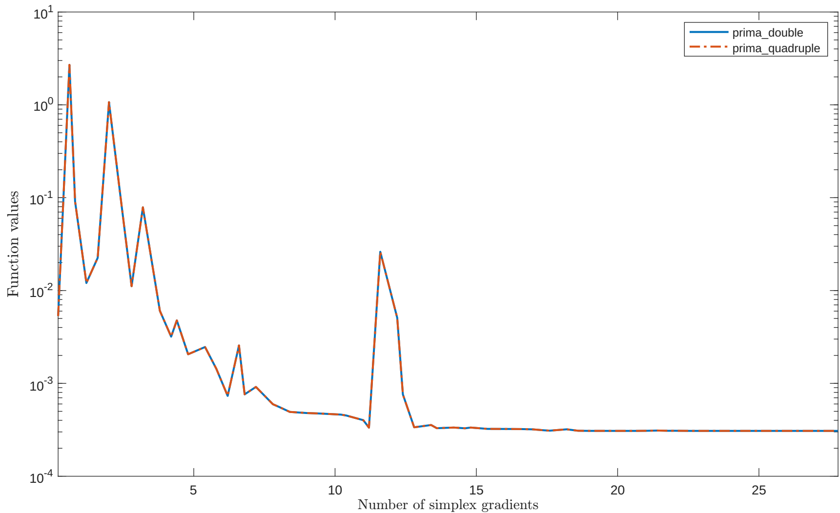
Solving “KOWOSB” with “plain” feature
