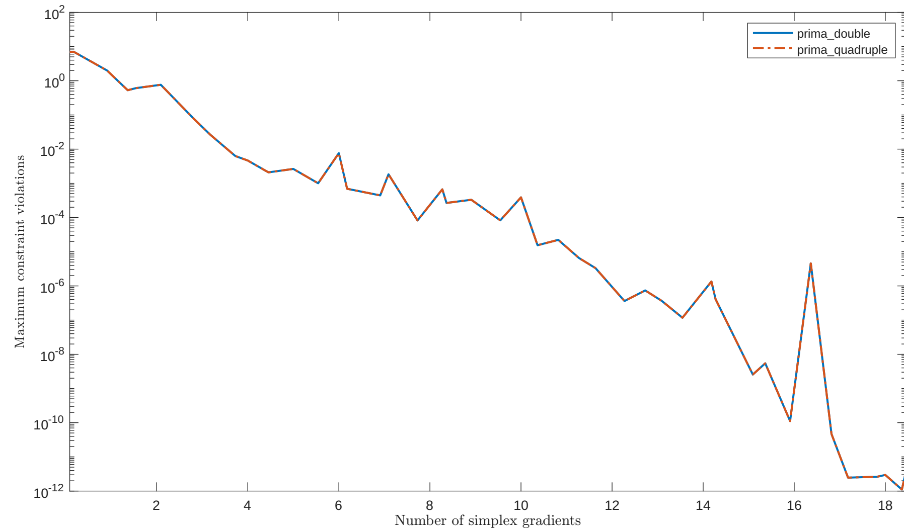
Solving "LUKVLE10" with "plain" feature
