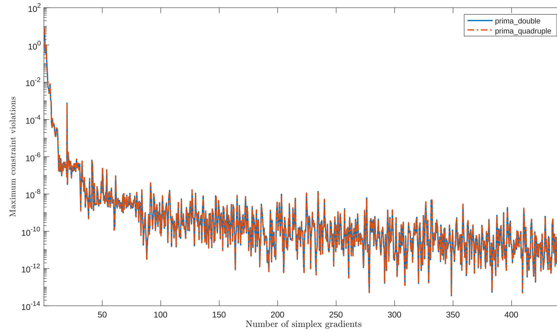
Solving "LUKVLE11" with "plain" feature
